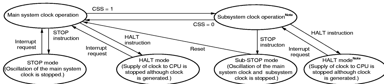
Figure 8-1. Standby Function
