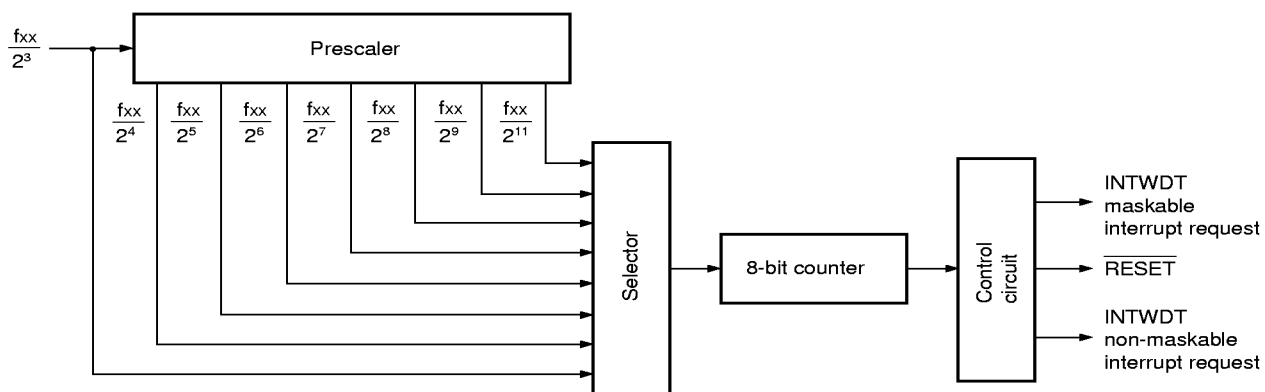
Figure 5-6. Watchdog Timer Block Diagram
