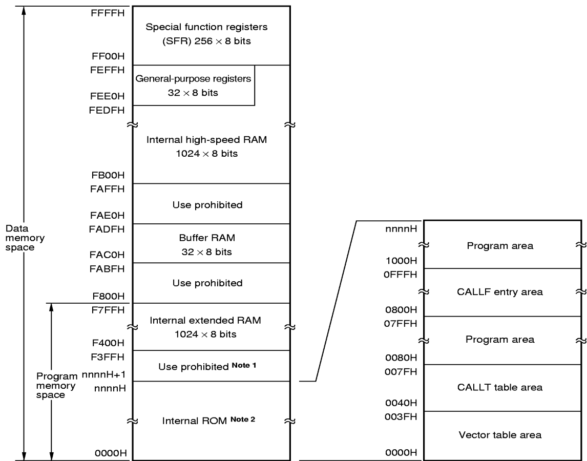
Figure 4-1. Memory Map
