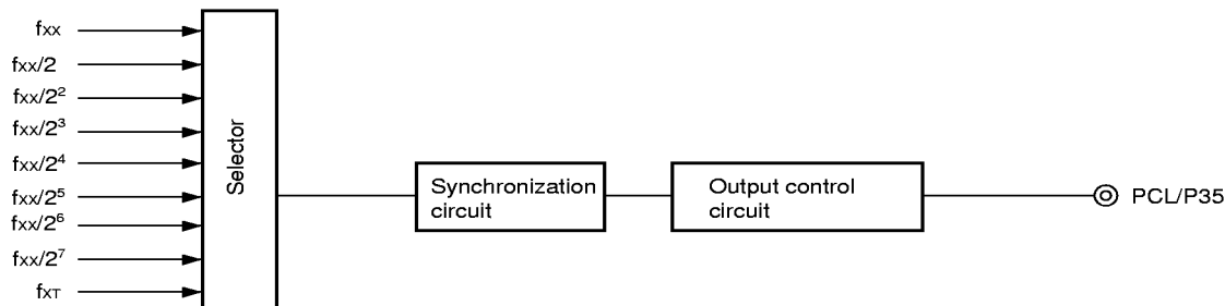
Figure 5-7. Clock Output Control Circuit Block Diagram
