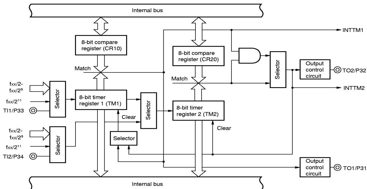
Figure 5-3. 8-Bit Timer/Event Counter 1, 2 Block Diagram
