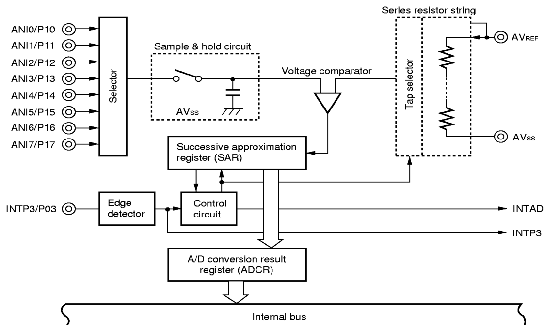
Figure 5-9. A/D Converter Block Diagram
