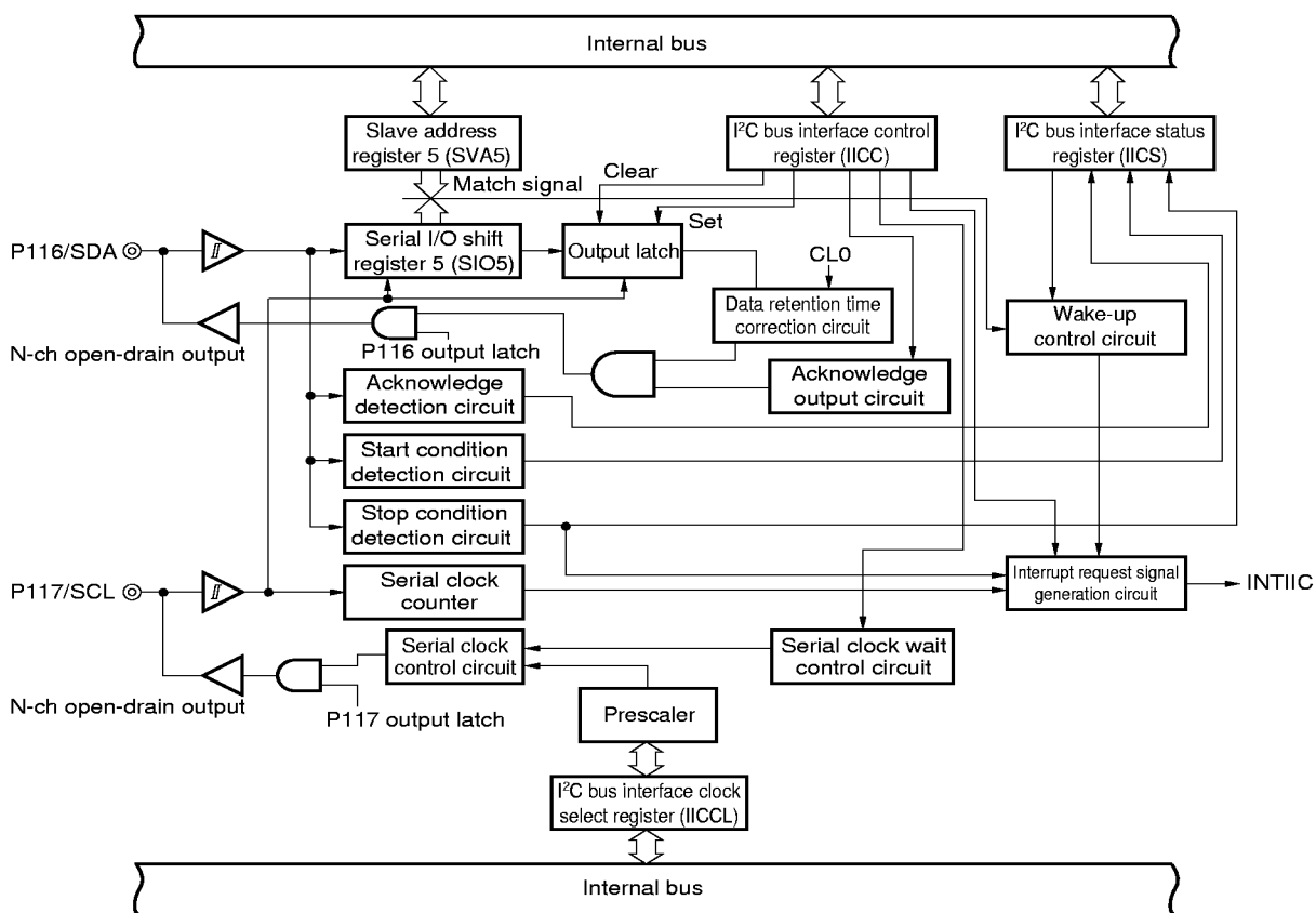
Figure 5-12. Serial Interface Channel 5 Block Diagram
