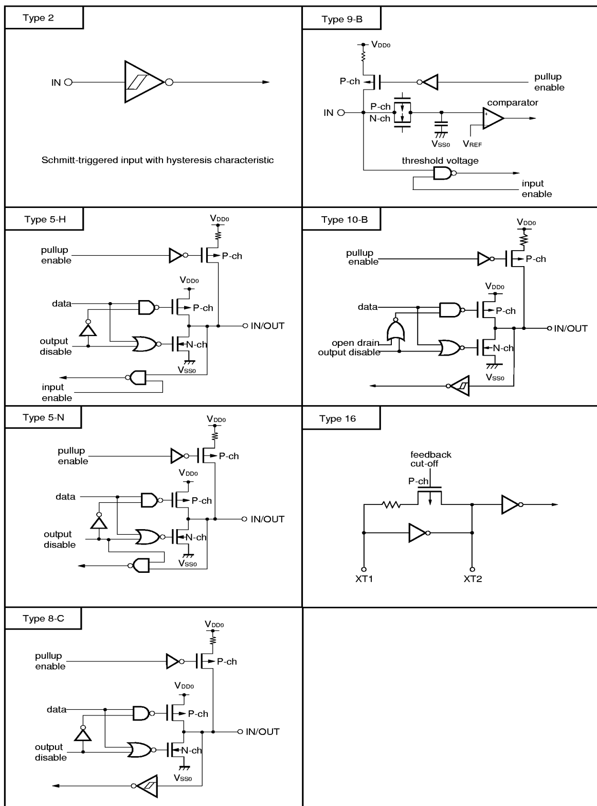
Figure 3-1. Pin Input/Output Circuits
