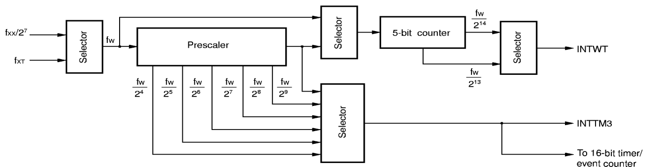
Figure 5-5. Watch Timer Block Diagram
