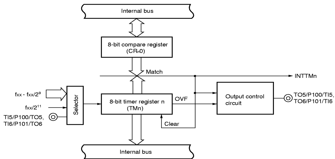
Figure 5-4. 8-Bit Timer/Event Counter 5, 6 Block Diagram
