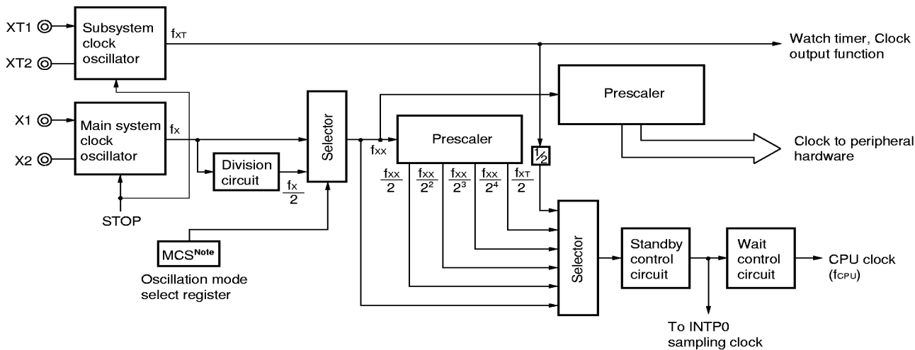
Figure 5-1. Clock Generator Block Diagram
