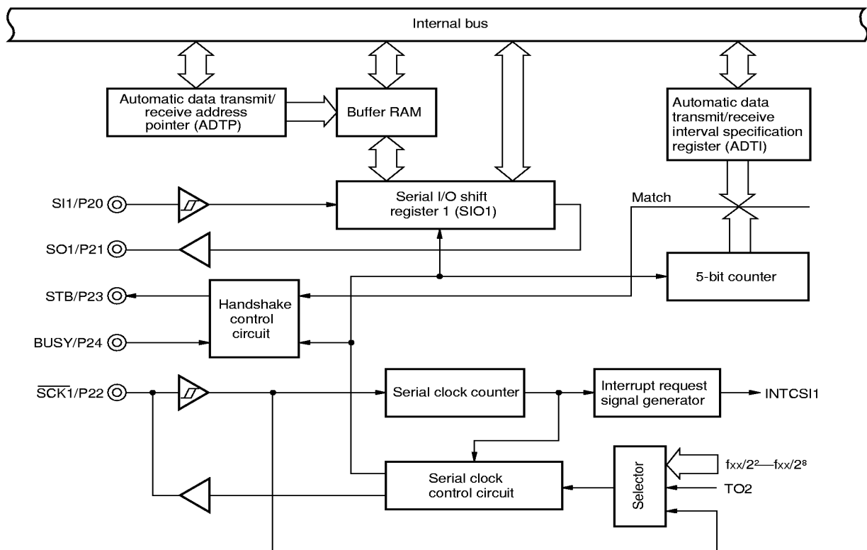
Figure 5-10. Serial Interface Channel 1 Block Diagram
