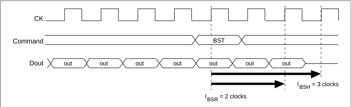
\overline{\text{CE}} Latency = 4, Burst Length = full page
