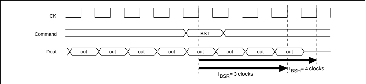
\overline{\text{CE}} Latency = 4, Burst Length = full page
