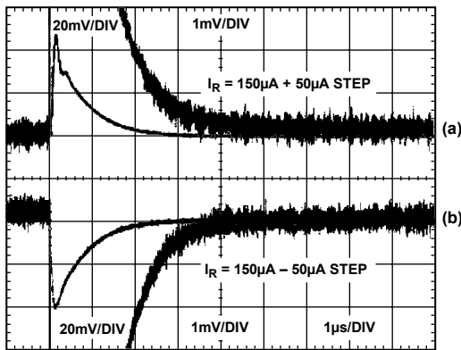
Figure 21. Transient Settling
