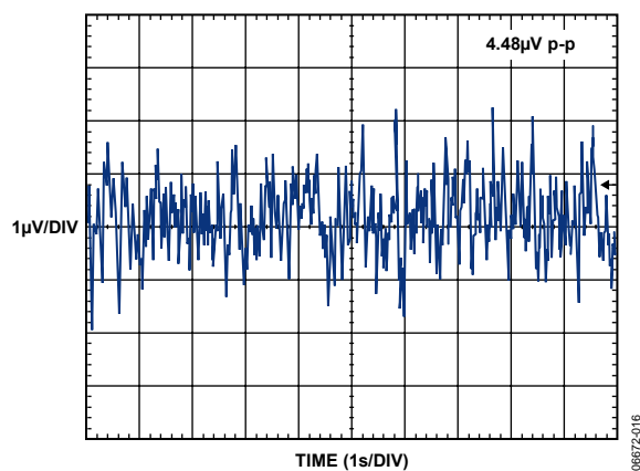
Figure 16. 0.1 Hz to 10 Hz Voltage Noise
