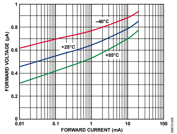
Figure 8. Forward Voltage vs. Forward Current
