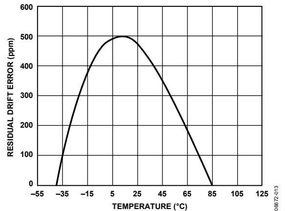
Figure 13. Residual Drift Error
