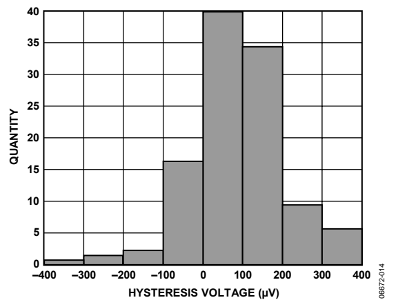
Figure 14. Reverse Voltage Hysteresis Distribution
