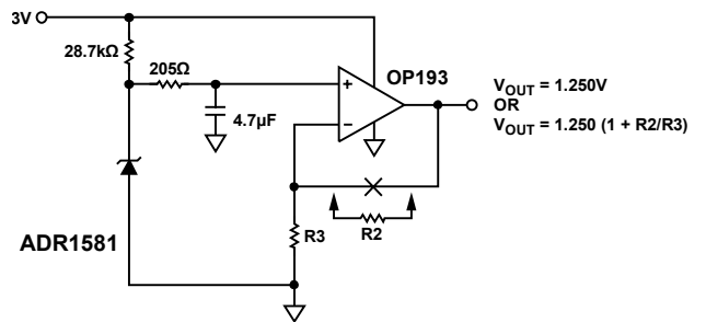
Figure 23. Micropower Buffered Reference
