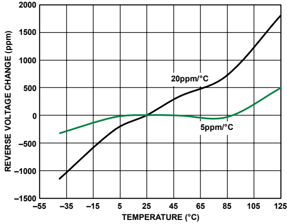
Figure 4. Output Drift for Different Temperature Characteristics
