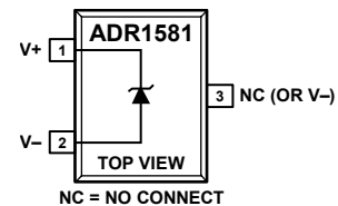
Figure 1. SOT-23
