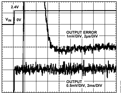
Figure 20. Turn-On Settling
