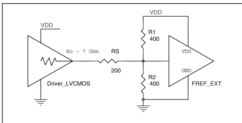
FIGURE 6C. EDGE RATE REDUCTION BY INCREASING THE RESISTOR VALUE
