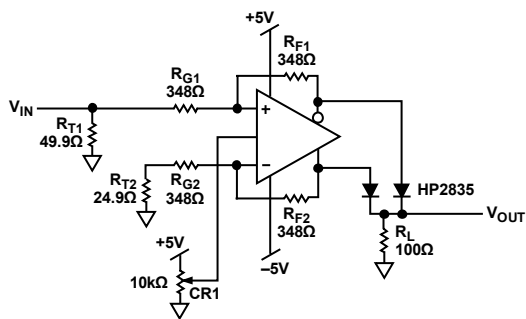
Figure 82. Full-Wave Rectifier
