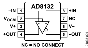
Figure 4. Pin Configuration
