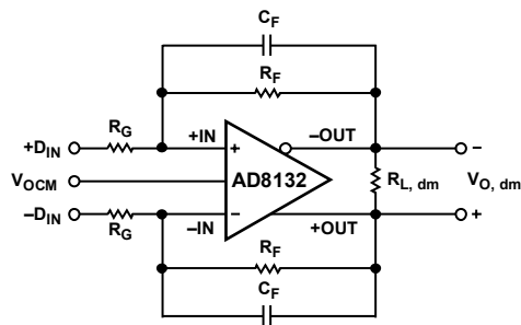
Figure 64. Circuit Definitions
