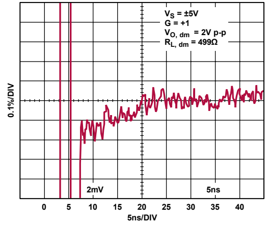
Figure 44. 0.1% Settling Time
