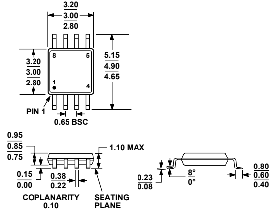
Figure 85. 8-Lead Mini Small Outline Package [MSOP] (RM-8) Dimensions shown in millimeters
