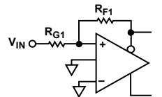
Figure 71. Typical Circuit with \beta_2 = 0
