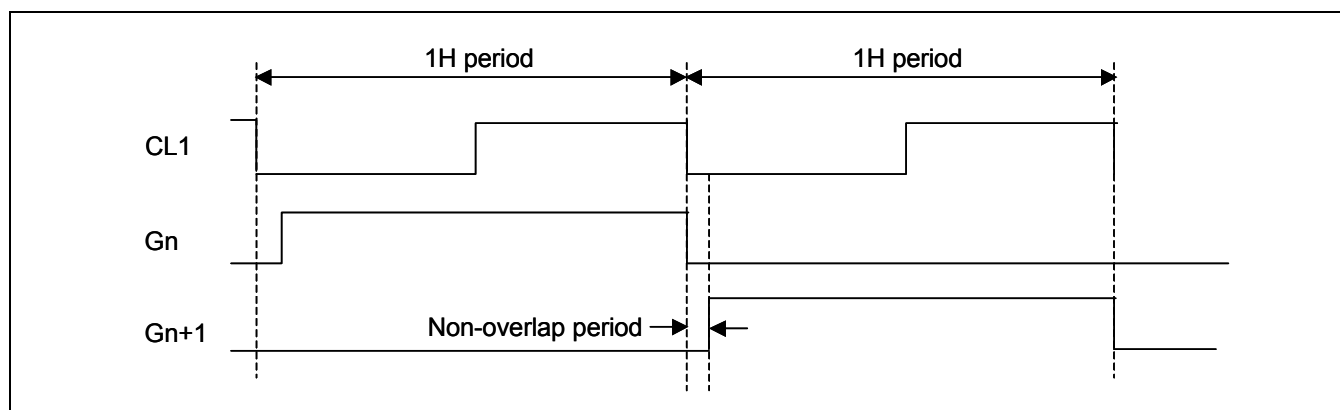
Figure 10. Non-overlap Period
