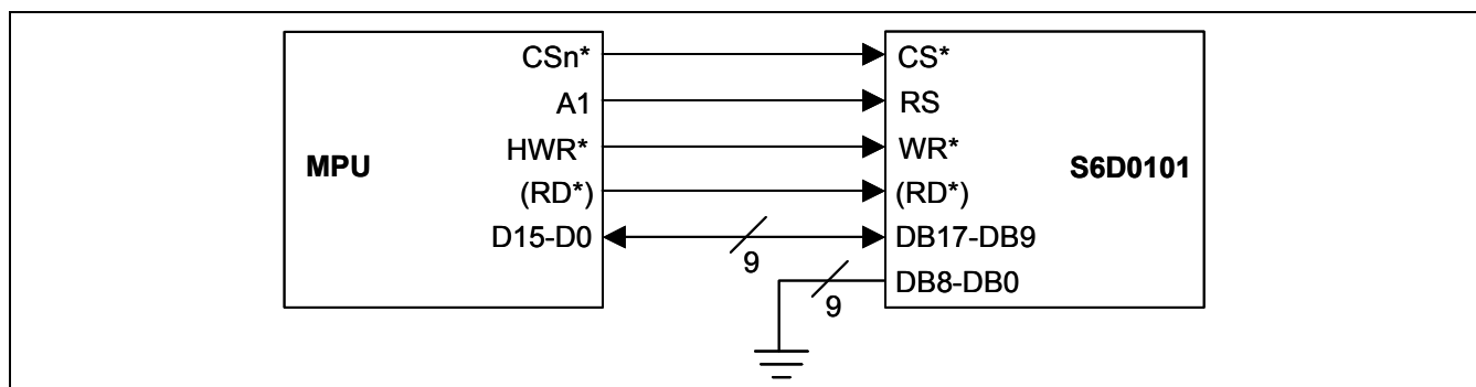
Figure 37. Interface to 9-bit Microcomputer
