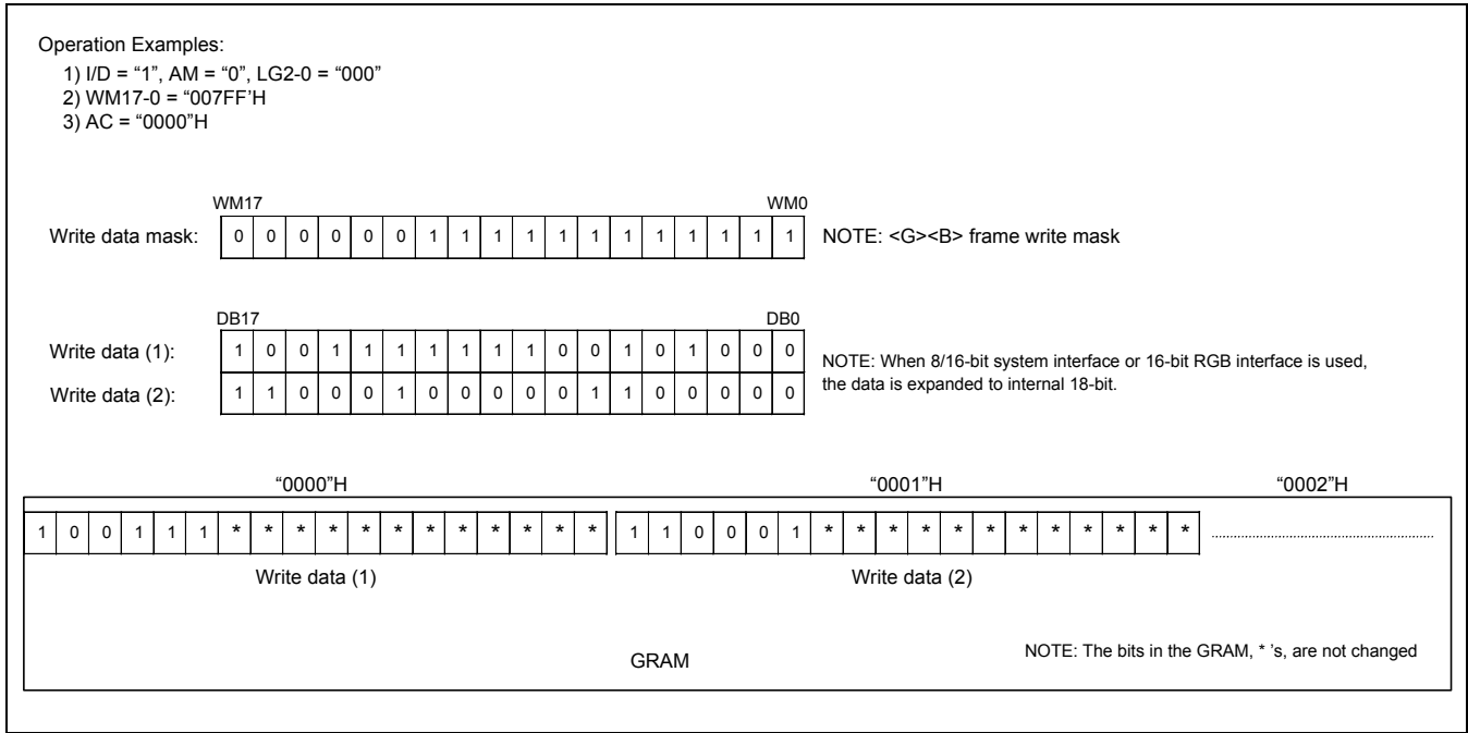
Figure 72. Writing operation of write mode 1
