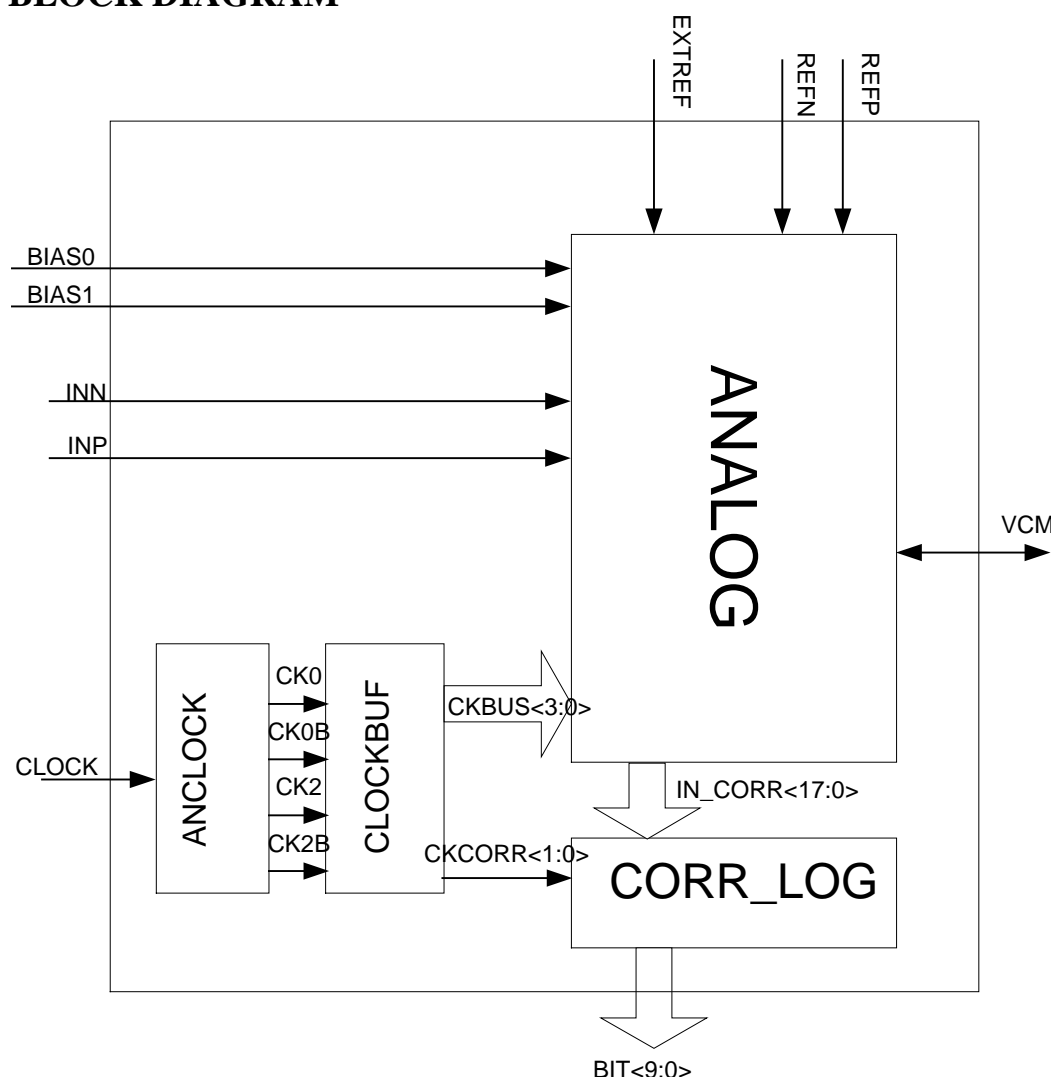
Figure 1. Block diagram nAD1040-18
