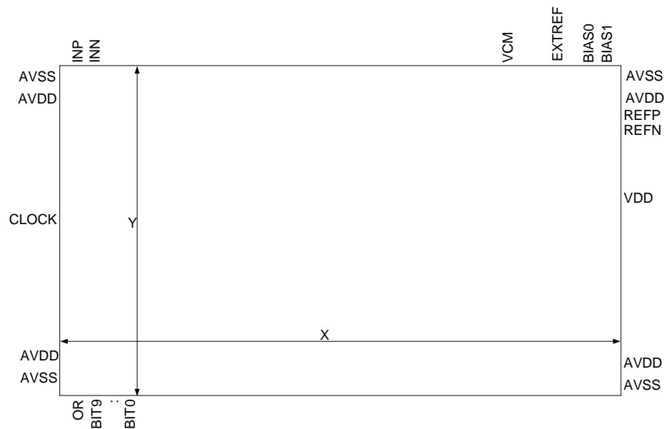
Figure 3. Size and pin placement for nAD1040-18.
