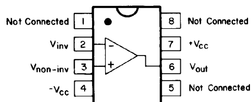
Pinout DIP & SOIC
