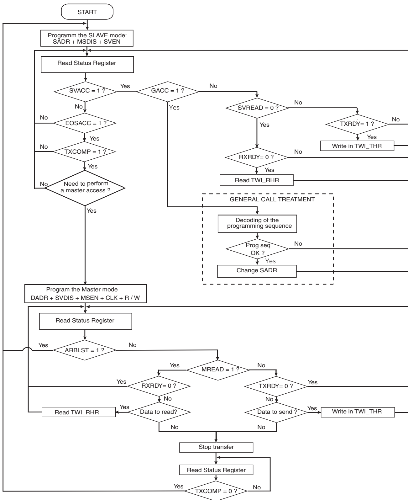
Figure 33-22. Multi-master Flowchart
