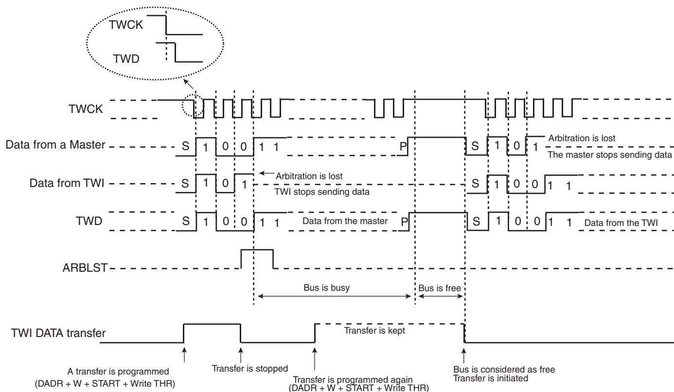
Figure 33-21. Arbitration Cases
