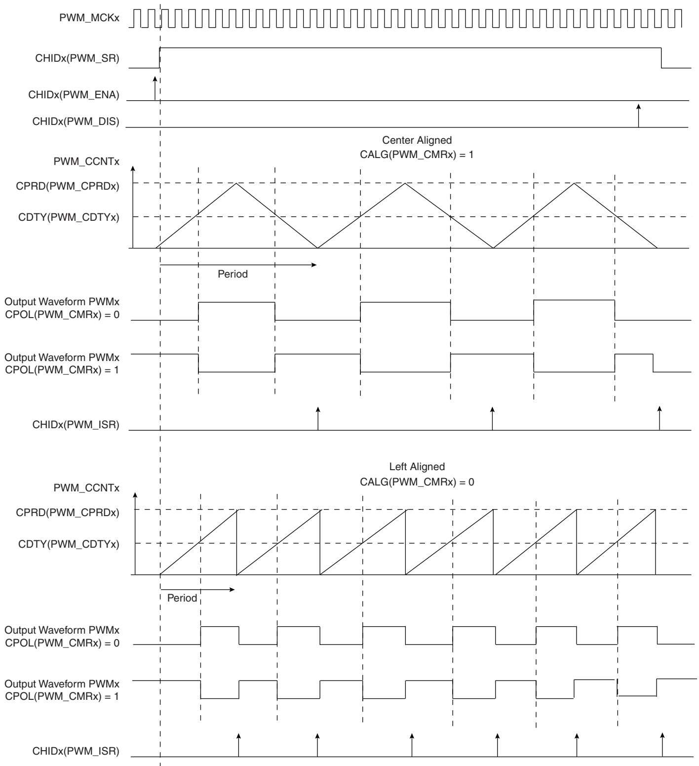
Figure 38-5. Waveform Properties
