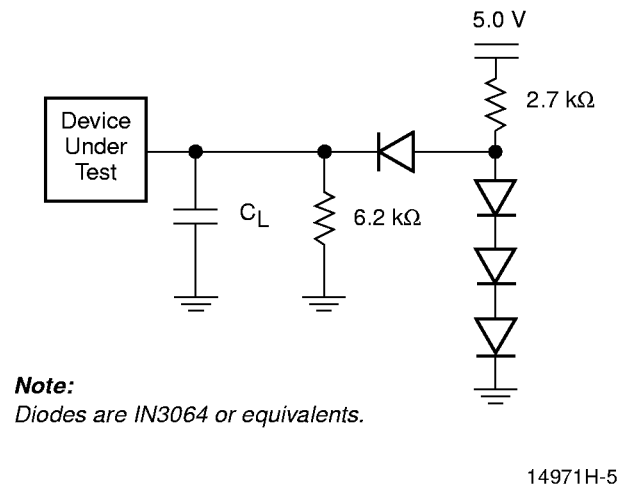
Figure 1. Test Setup
