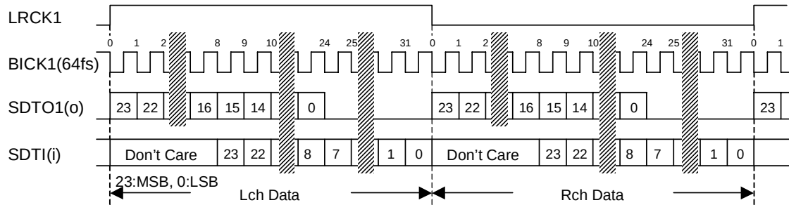
Figure 2. Mode 1,5 Timing
