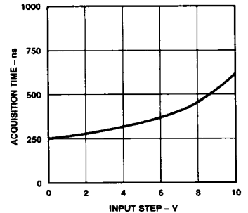
Acquisition Time (to 0.01%) vs. Input Step Size
