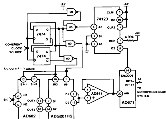
Figure 10. The AD682 Used for I and Q Demodulation
