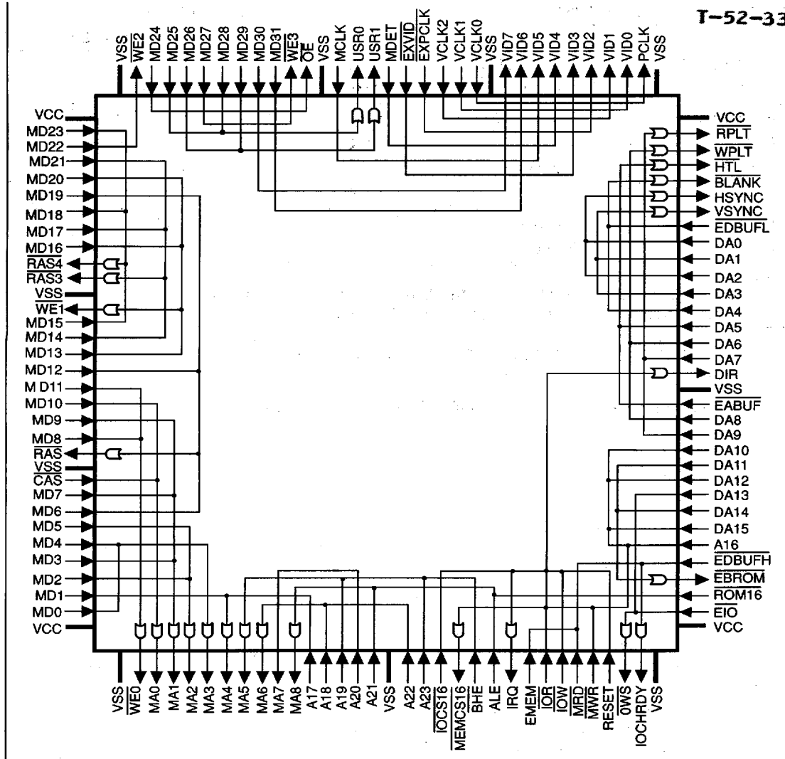
FIGURE 26. WD90C30 PIN SCAN MAP FOR A 132-PIN PACKAGE
