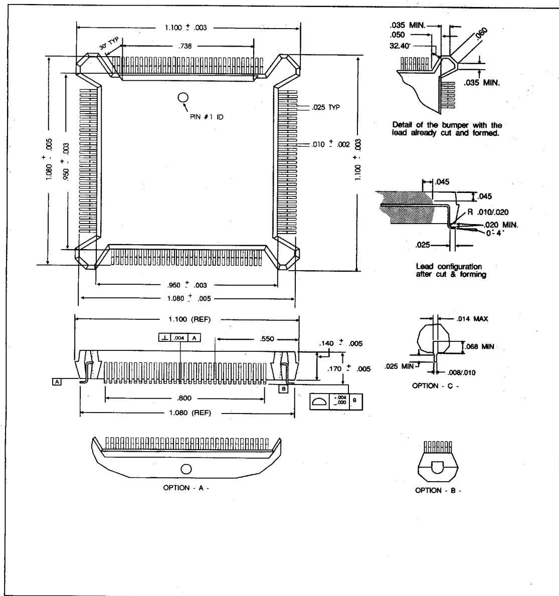
FIGURE 27. 132-PIN PQFP PACKAGE DIMENSIONS
