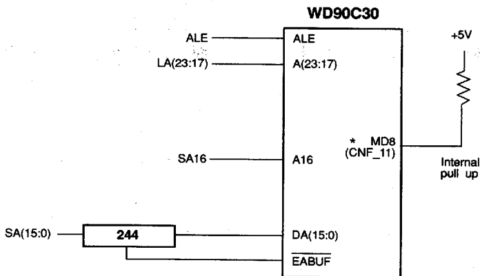
16 BIT INTERFACE (Versions A and B)
