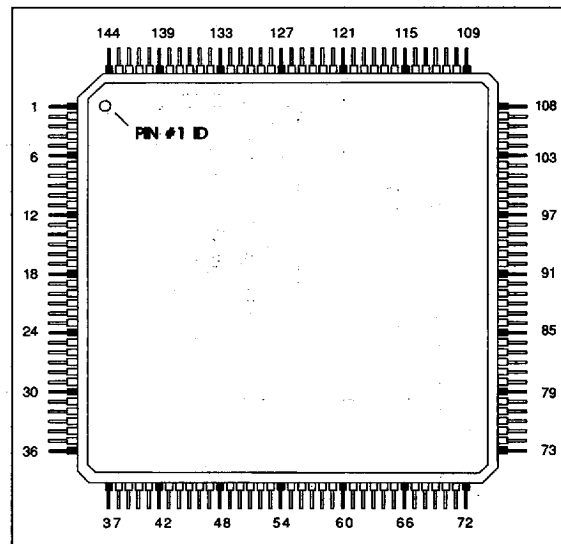
FIGURE 4. 144-PIN MQFP PACKAGE
