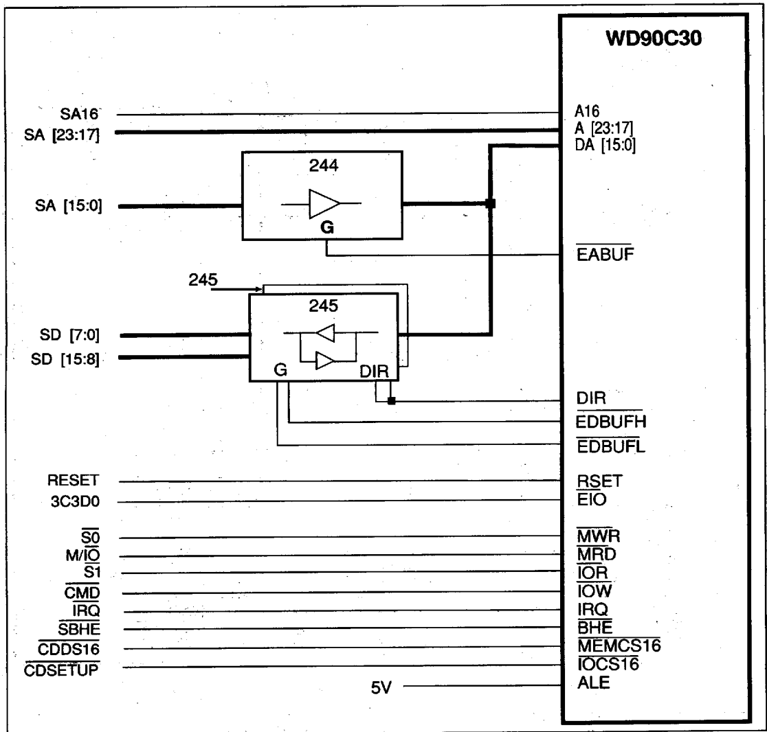
FIGURE 17. 16-BIT MICRO CHANNEL INTERFACE
