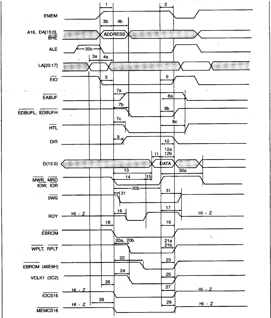
FIGURE 7. AT MODE BUS TIMING
