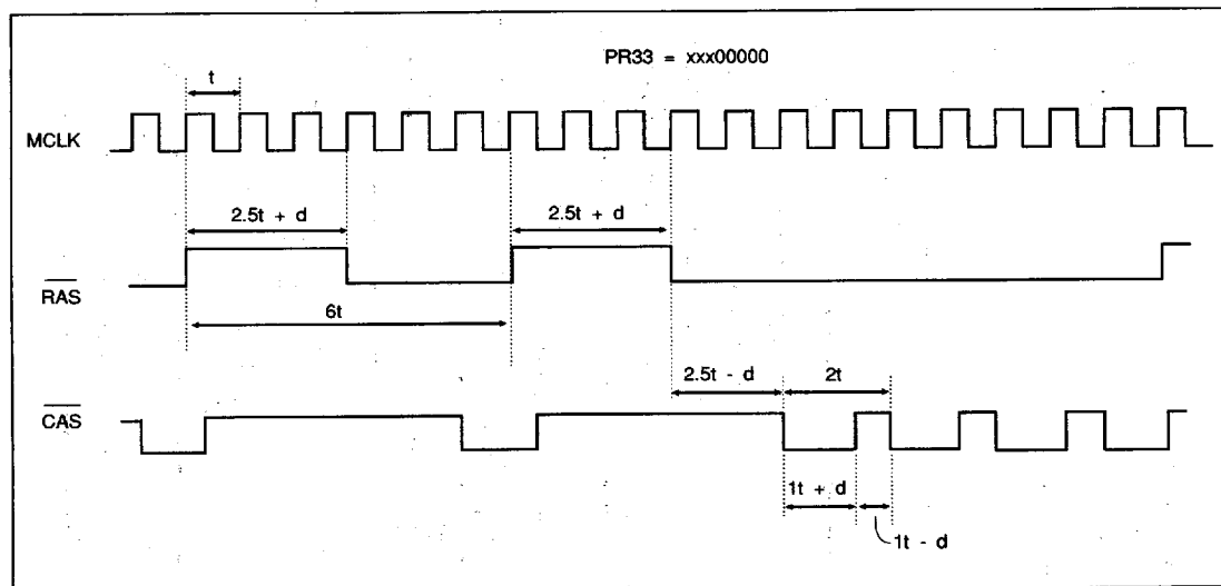
FIGURE 11. 256K BY 4 DRAM TIMING
