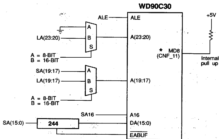
8 OR 16 BIT INTERFACE (Version B)
