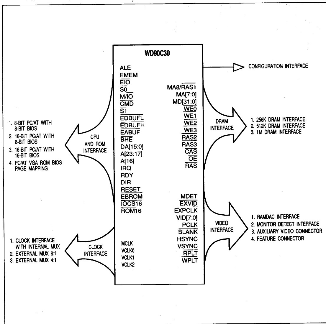
FIGURE 13. WD90C30 INTERFACES
