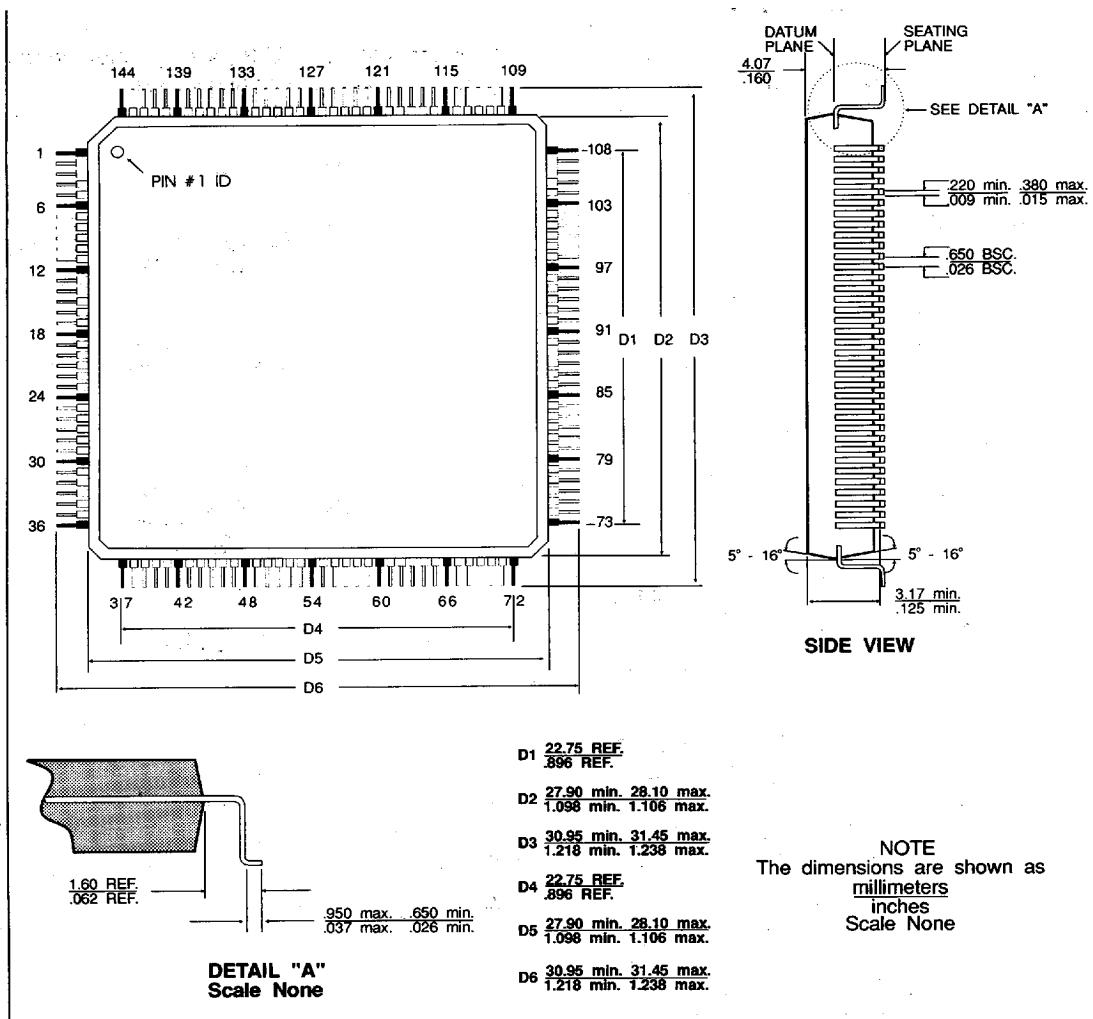
FIGURE 28. 144-PIN MQFP PACKAGE DIMENSIONS
