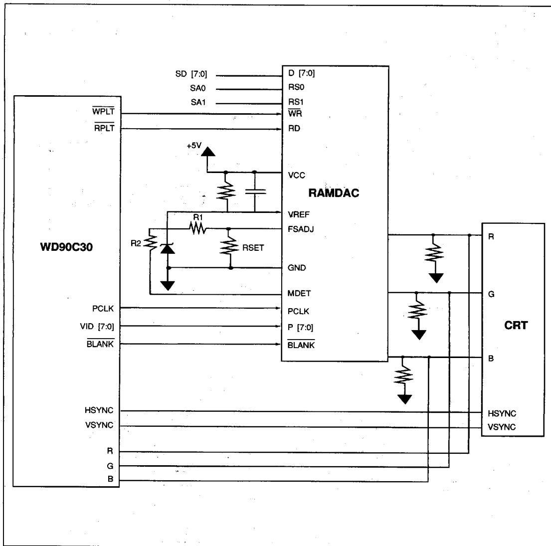
FIGURE 21. WD90C30 WITH RAMDAC INTERFACE
