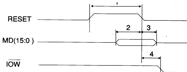
FIGURE 5. RESET TIMING
