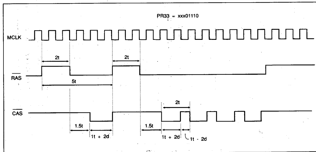
FIGURE 12. 64K BY 16 DRAM TIMING
