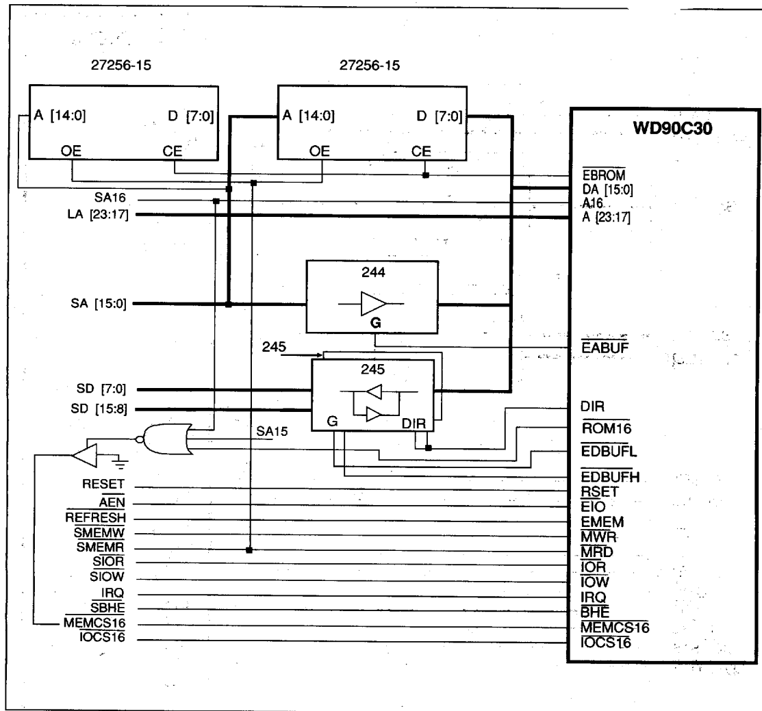
FIGURE 16. 16-BIT PC AT INTERFACE WITH 16-BIT BIOS
