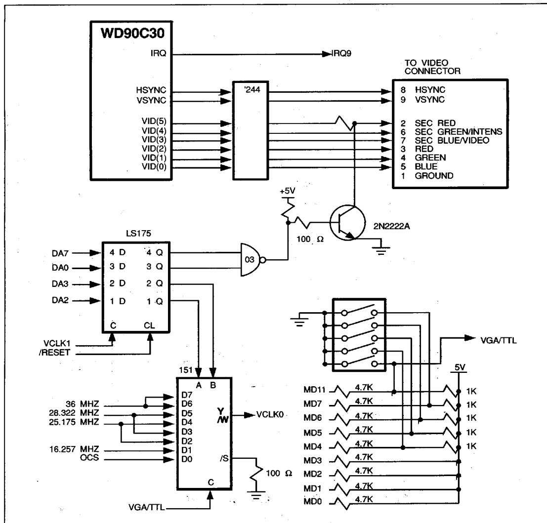
FIGURE 22. WD90C30 AND TTL MONITOR CONNECTIONS
