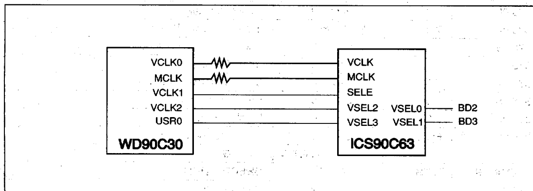
FIGURE 23. CLOCK INTERFACE
