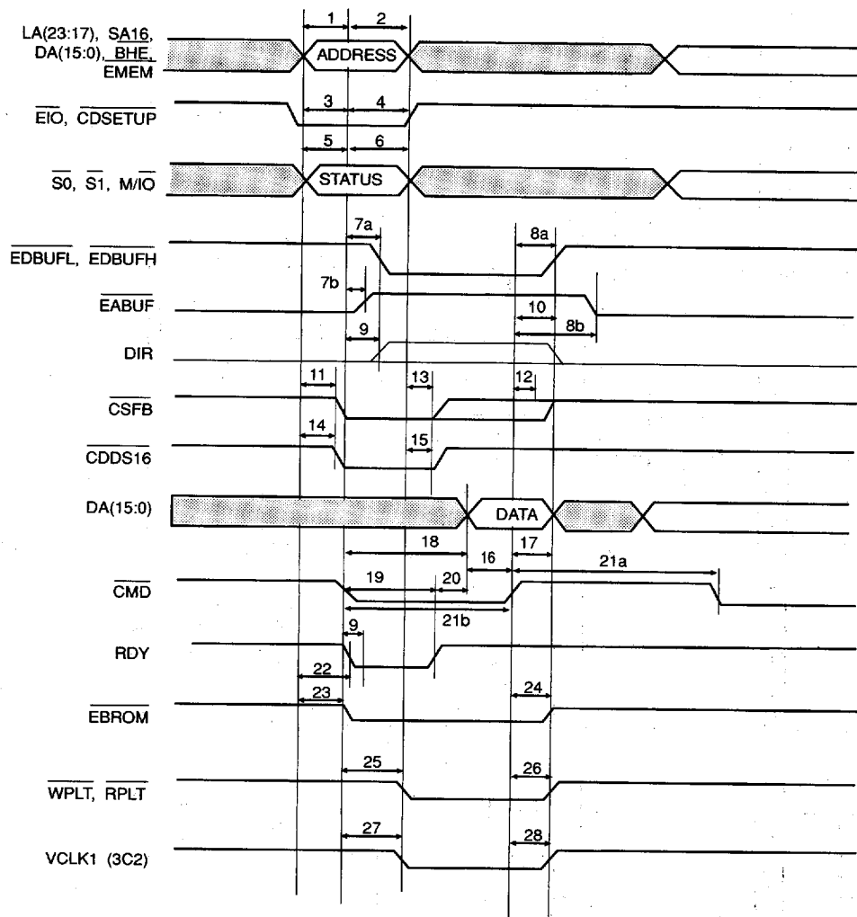
FIGURE 8. MICRO CHANNEL MODE BUS TIMING
