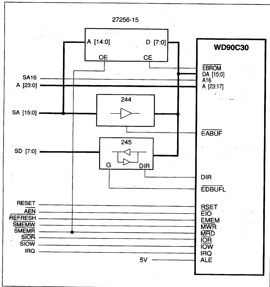
FIGURE 14. 8-BIT PC AT INTERFACE WITH 8-BIT BIOS
