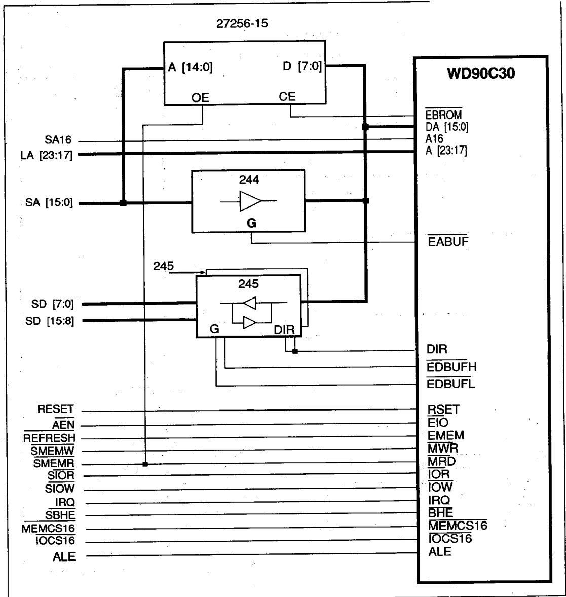
FIGURE 15. 16-BIT PC AT INTERFACE WITH 8-BIT BIOS
