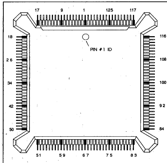
FIGURE 3. 132-PIN PQFP PACKAGE
