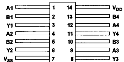
14-Pin Flatpack Top View
