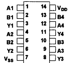
14-Pin Flatpack Top View
