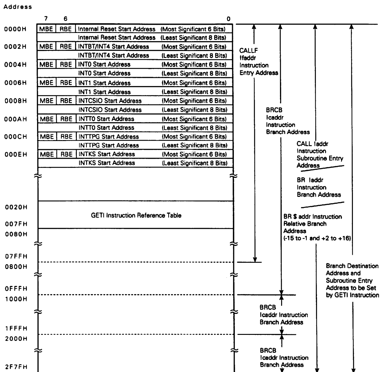
Fig. 4-1 Program Memory Map
