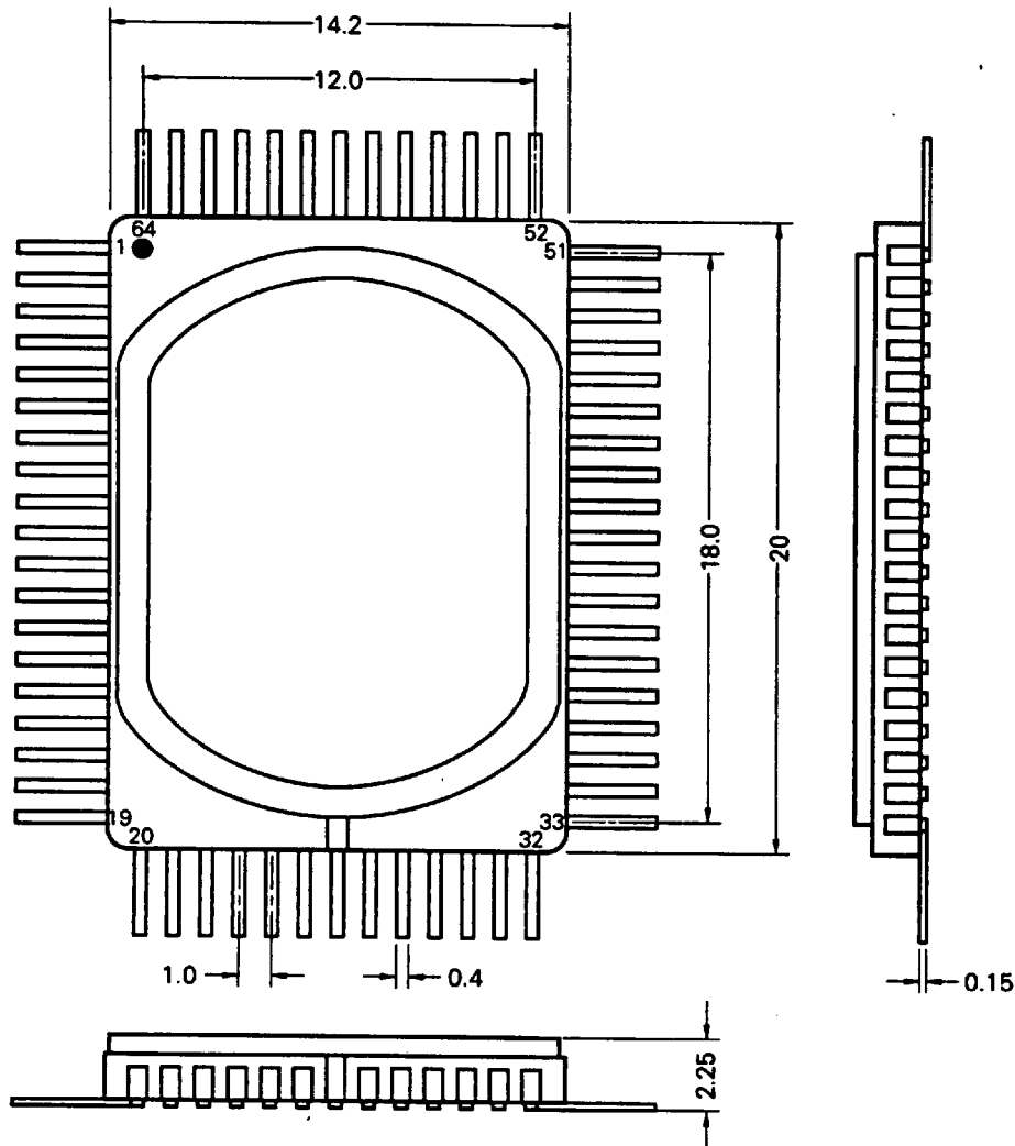
64-pin ceramic QFP for ES (reference) (unit : mm)
