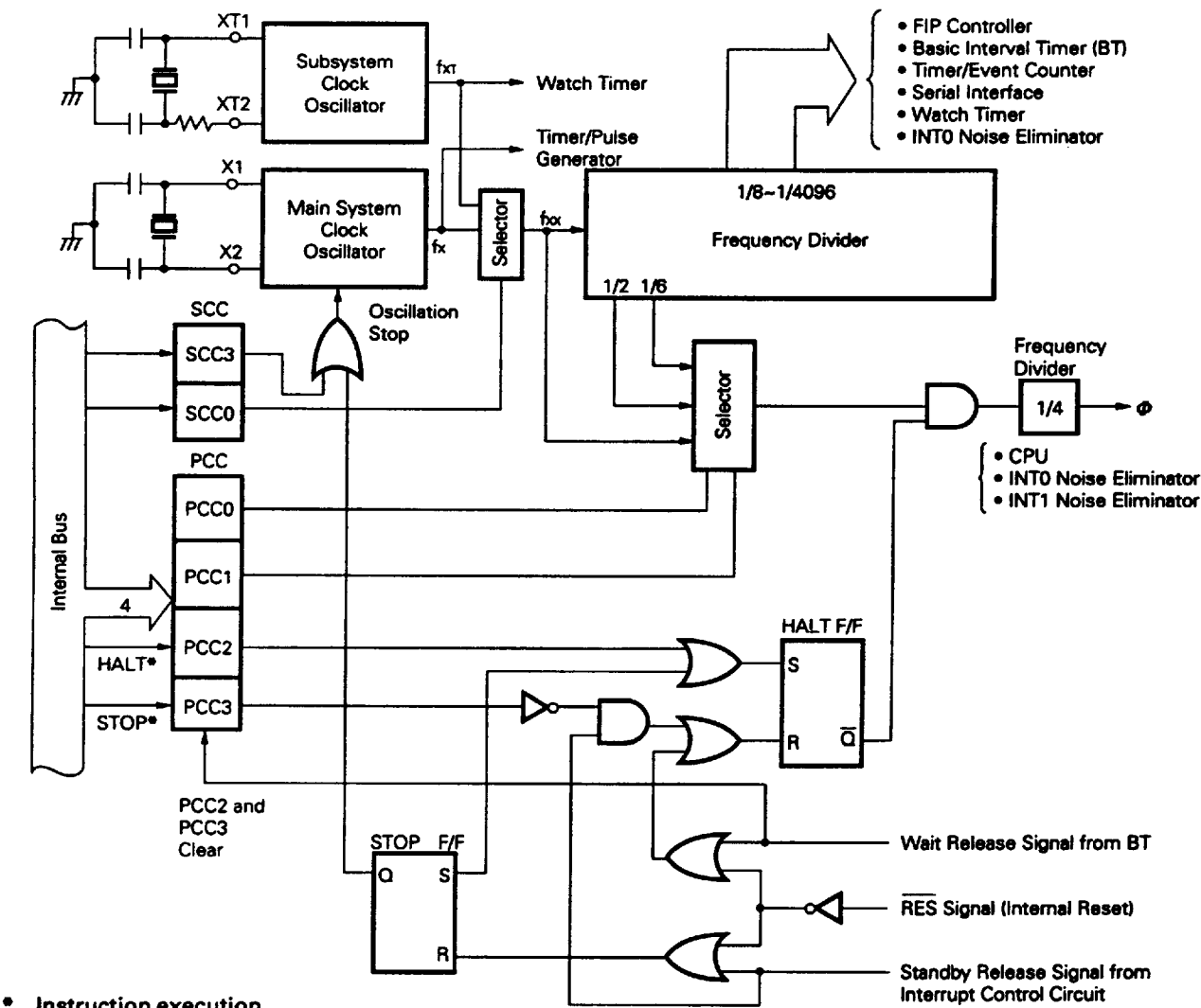
Fig. 5-1 Clock Generator Block Diagram
