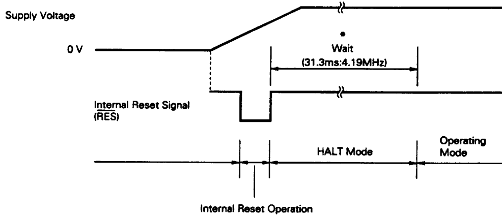
Fig. 8-2 Reset Operation by Power-On Reset
