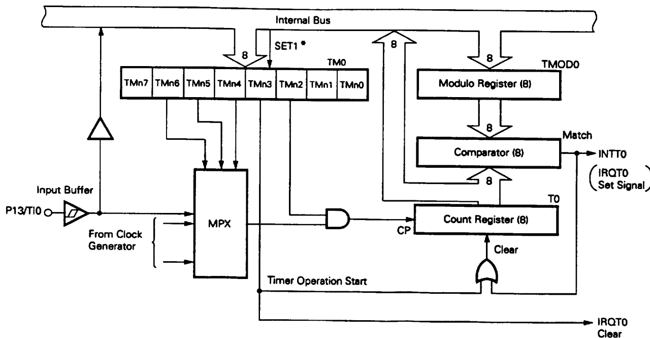
Fig. 5-4 Timer/Event Counter Block Diagram
