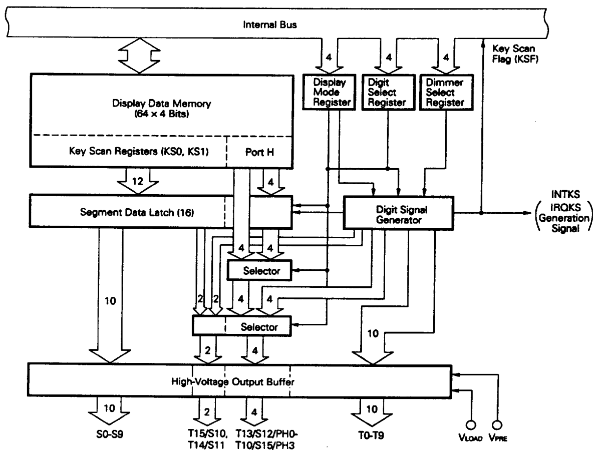
Fig. 5-8 FIP Controller/Driver Block Diagram
