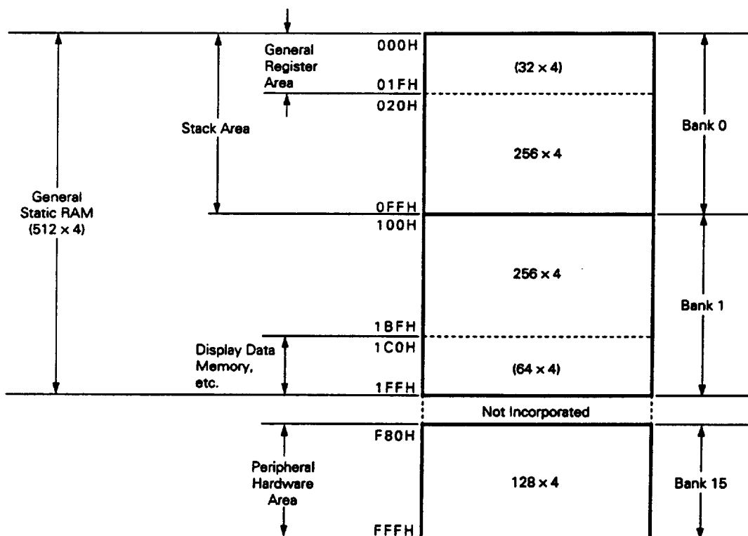
Fig. 4-2 Data Memory Map
