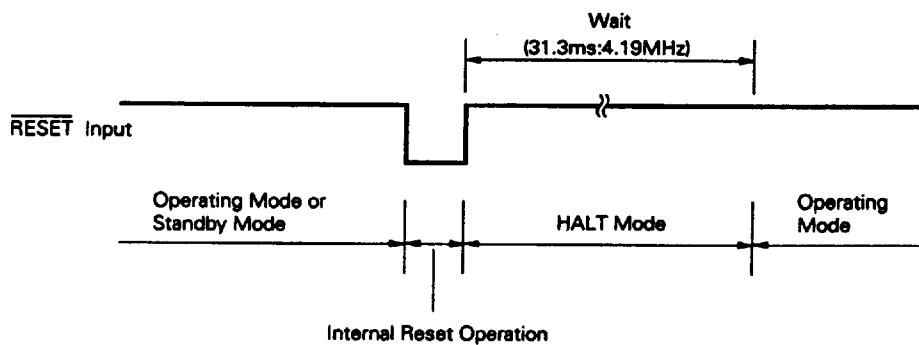
Fig. 8-3 Reset Operation by \overline{RESET} Input
