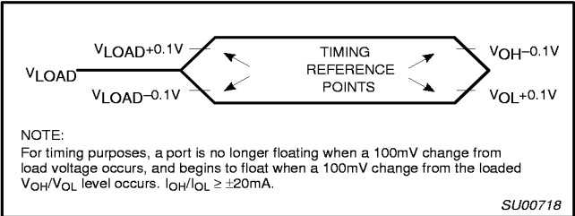
Figure 20. Float Waveform
