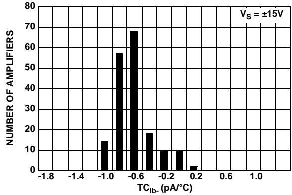
FIGURE 14. TC_{1b-} vs NUMBER OF AMPLIFIERS, V_S = \pm 15V
