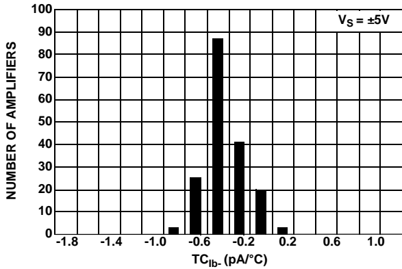
FIGURE 13. TC_{1b-} vs NUMBER OF AMPLIFIERS, V_S = \pm 5V
