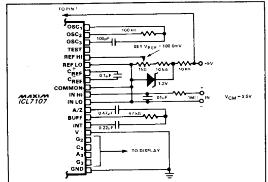
Figure 18. ICL7107 Operated from Single +5V Supply. An external Reference must be used in this application.
