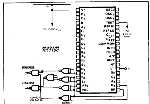
Figure 16. Circuit for Developing Under Range and Over Range Signals from ICL7106 Outputs.
