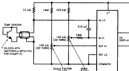
Figure 20. Digital Thermometer
