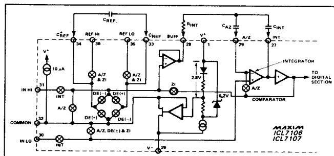
Figure 3. Analog Section of ICL7106/ICL7107
