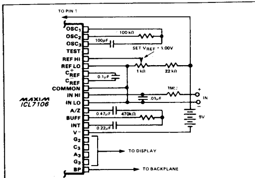
Figure 13. ICL7106 using the Internal Reference. 2V Full Scale; 3 Readings per Second.
