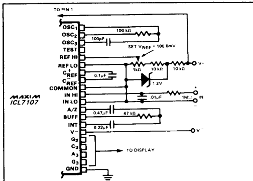
Figure 17. ICL7107 with a 1.2V External Band-Gap Reference V_{IN} tied to common.
