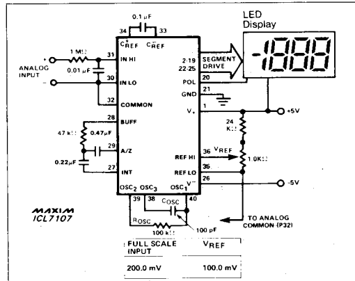
Figure 2. Maxim ICL7107 Typical Operating Circuit
