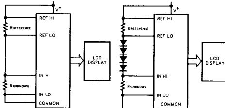
ICL7106 system setup for 2V reference
