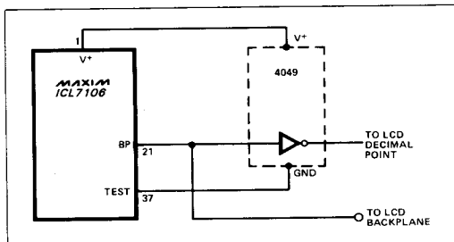
Figure 5A. Fixed Decimal Point Drivers
