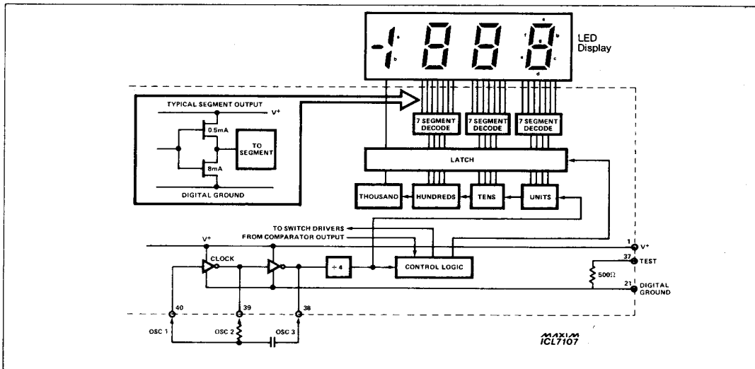
Figure 9. ICL7107 Digital Section
