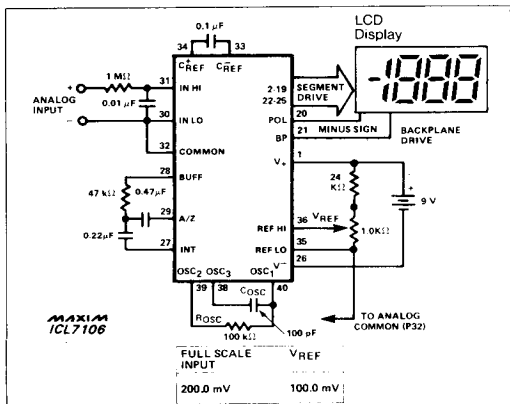
Figure 1. Maxim ICL7106 Typical Operating Circuit
