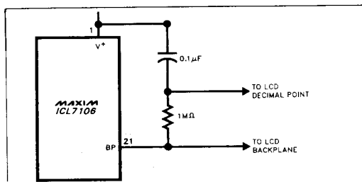
Figure 5B. Fixed Decimal Point Drivers
