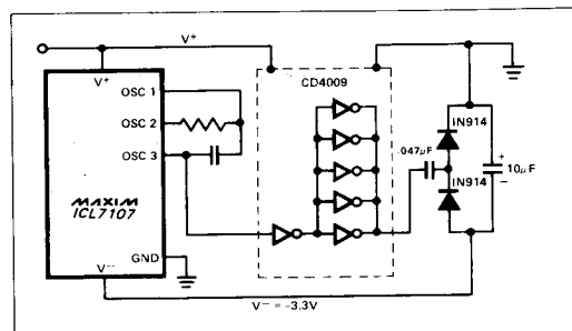
Figure 10. Generating Negative Supply from +5V
