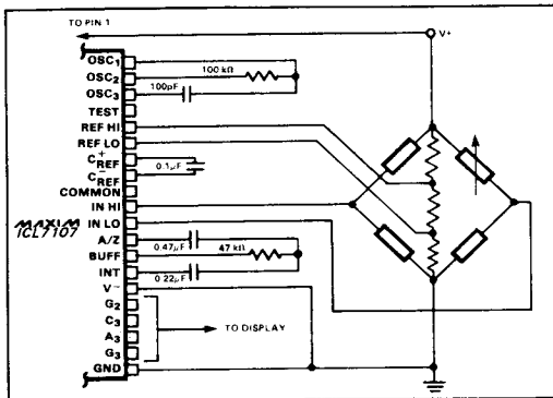
Figure 15. ICL7107 Measuring Ratiometric Values of a Load Cell. Desired Sensitivity is Determined by Resistor Values Within the Bridge.
