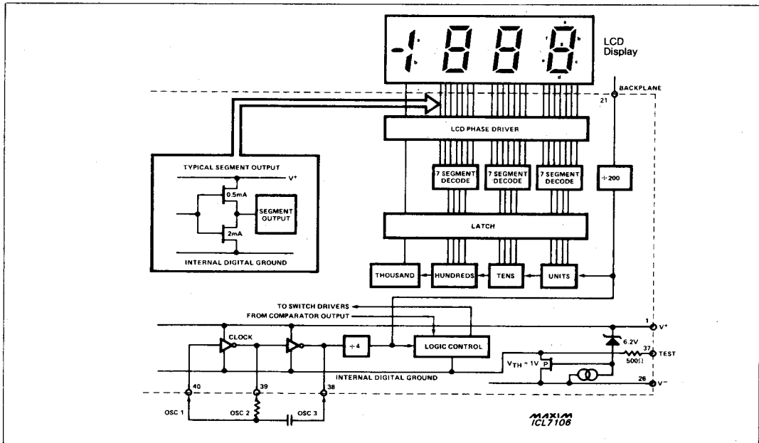
Figure 8. ICL7106 Digital Section
