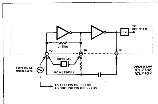
Figure 7. Clock Circuits
