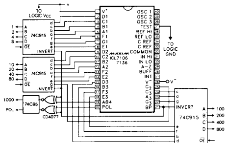
Figure 21. BCD Output from 7-Segment Drivers
