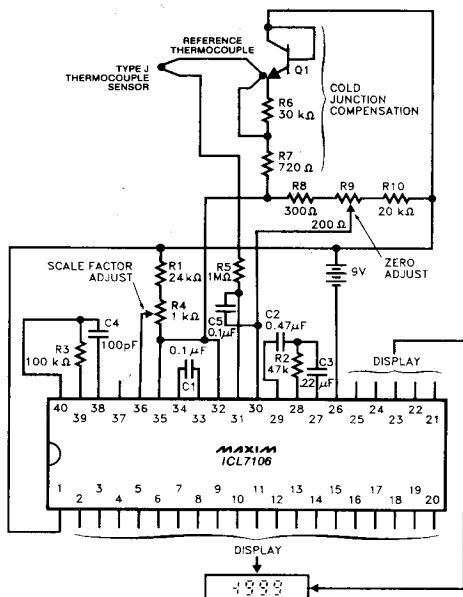
Figure 19. Thermocouple Thermometer. This circuit operates with approximately 50mV reference, so the 50.4μV/°C output of a Type J thermocouple results in 1 count/°C.
