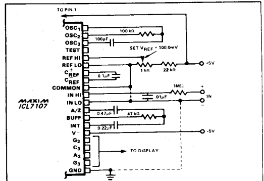
Figure 14. ICL7107 Internal Reference. 200mV Full Scale; 3 Readings per Second, V_{IN} Tied to GND for Single Ended Inputs. (See discussion under "Analog Common".)
