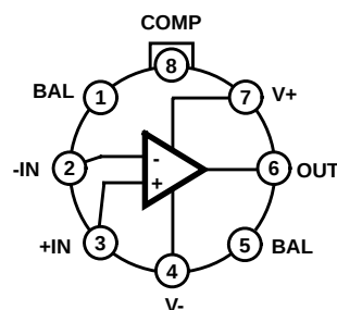
HA-2600/883, HA-2602/883 (METAL CAN) TOP VIEW
