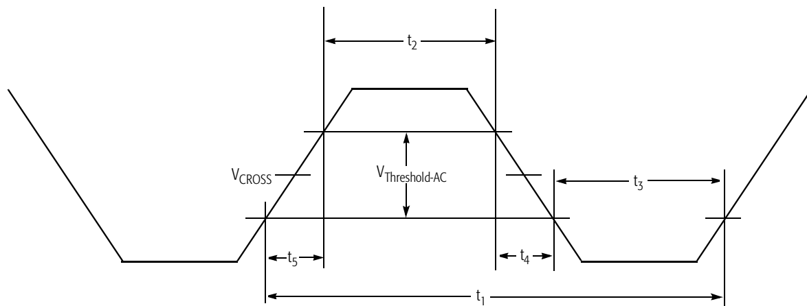
Figure 9. SYSCLK Waveform
