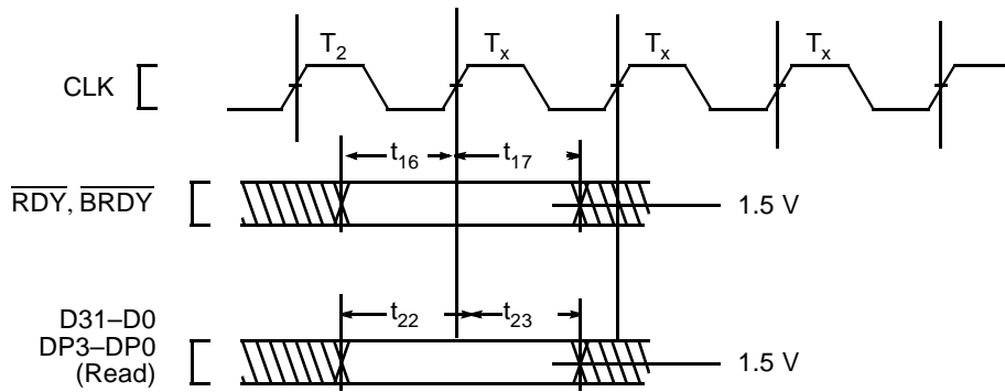
Figure 5. RDY and BRDY Input Setup and Hold Timing
