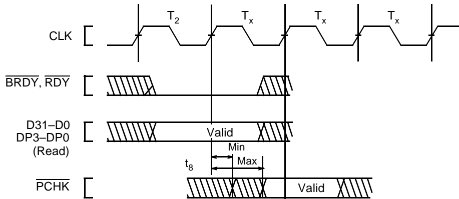
Figure 6. PCHK Valid Delay Timing
