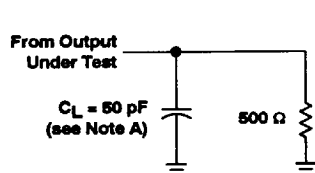
LOAD CIRCUIT
