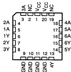
54AC11004 ... FK PACKAGE (TOP VIEW)
