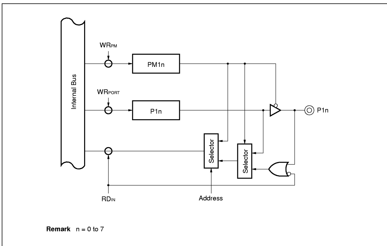
Figure 9-3. Block Diagram of P10 to P17 (Port 1)
