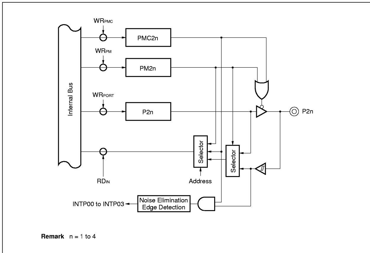
Figure 9-5. Block Diagram of P21 to P24 (Port 2)
