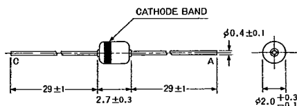
Fig. 1 Glass sealed mini-package JEDEC: DO-34
