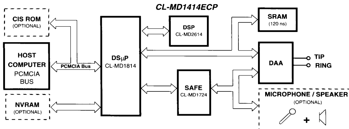
CL-MD1414ECP Functional Block Diagram
