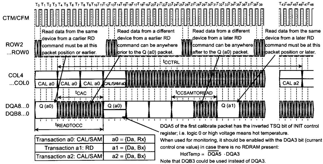
Figure 39. Current Control CAL/SAM transaction Example
