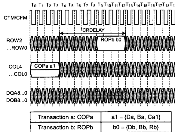
Figure 10. COL-to-ROW Packet Interaction Timing
