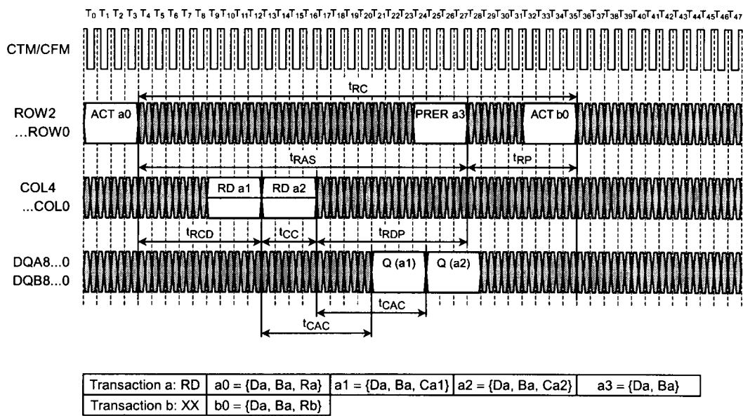
Figure 16. Read Transaction Example
