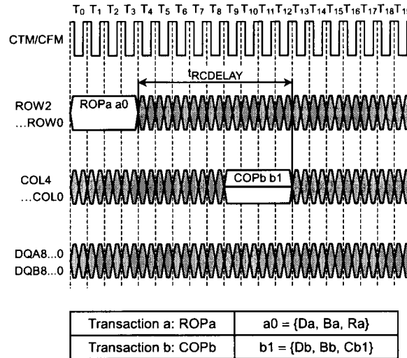
Figure 8. ROW-to-COL Packet Interaction Timing
