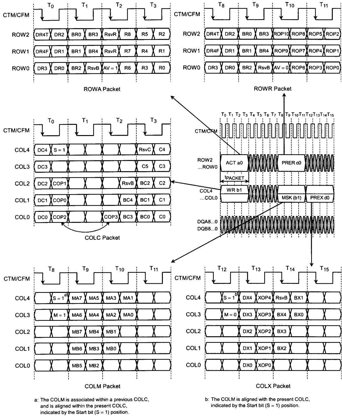
Figure 4. Packet Formats
