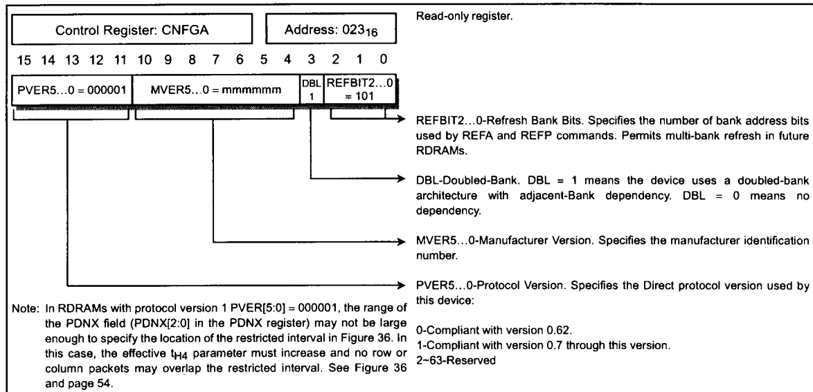
Figure 28. Control Registers
