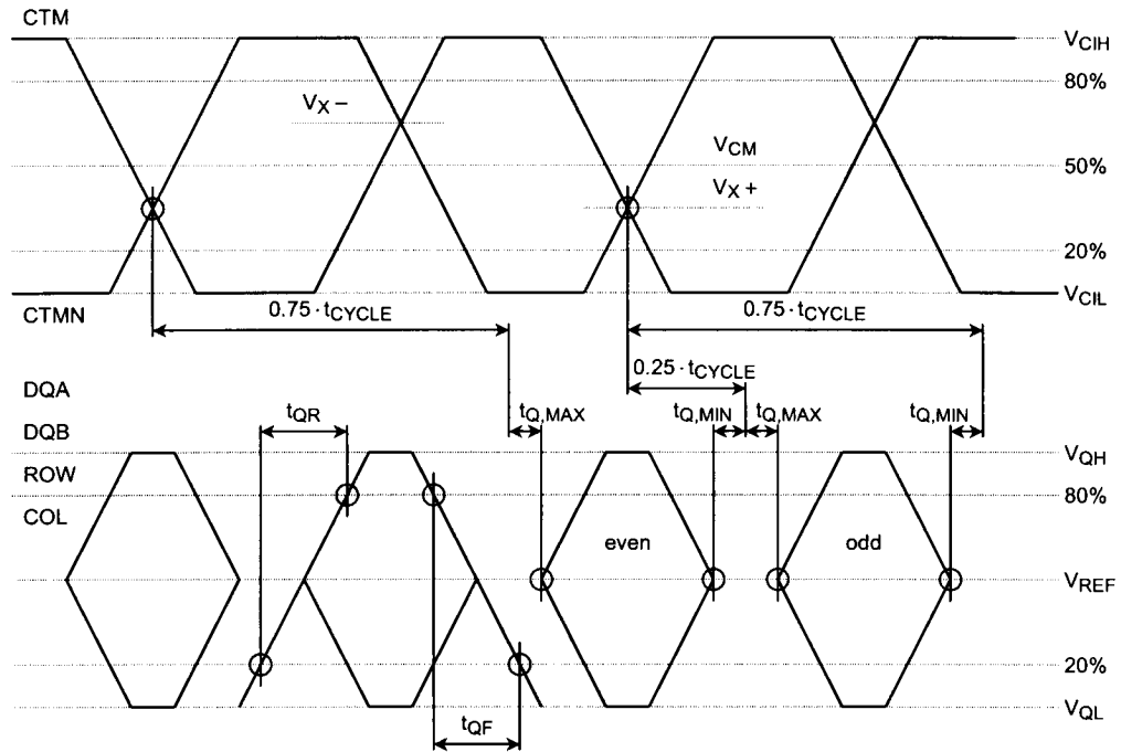
Figure 43. RSL Timing-Data Signals for Transmit
