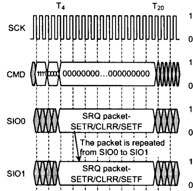
Figure 26. SETR, CLRR, SETF Transaction
