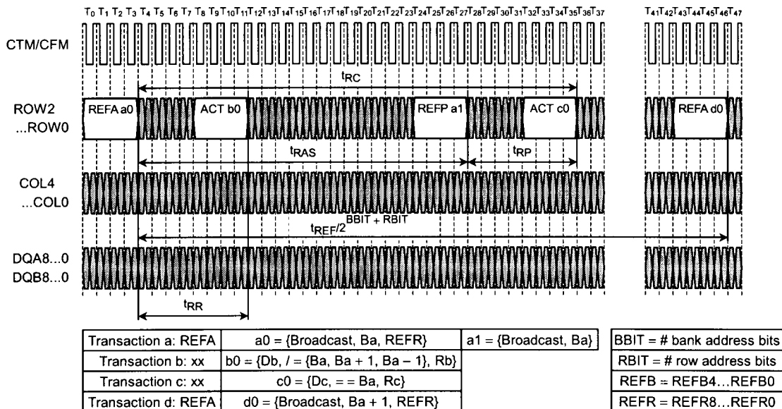
Figure 38. REFA/REFP Refresh Transaction Example
