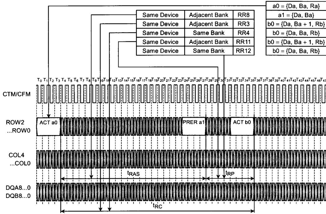
Figure 11. ROW Packet Example
