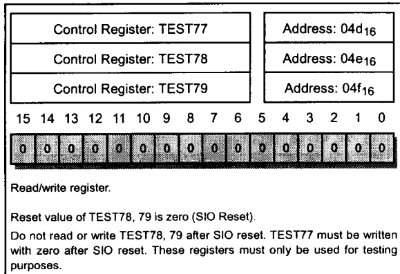
Figure 32. Control Registers
