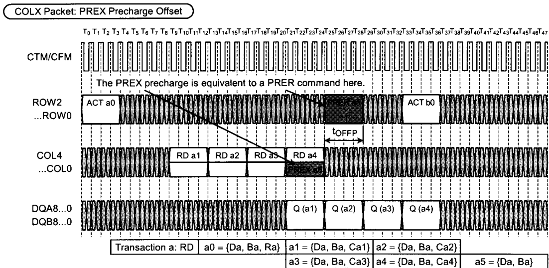
Figure 15. Offsets for Alternative Precharge Mechanisms
