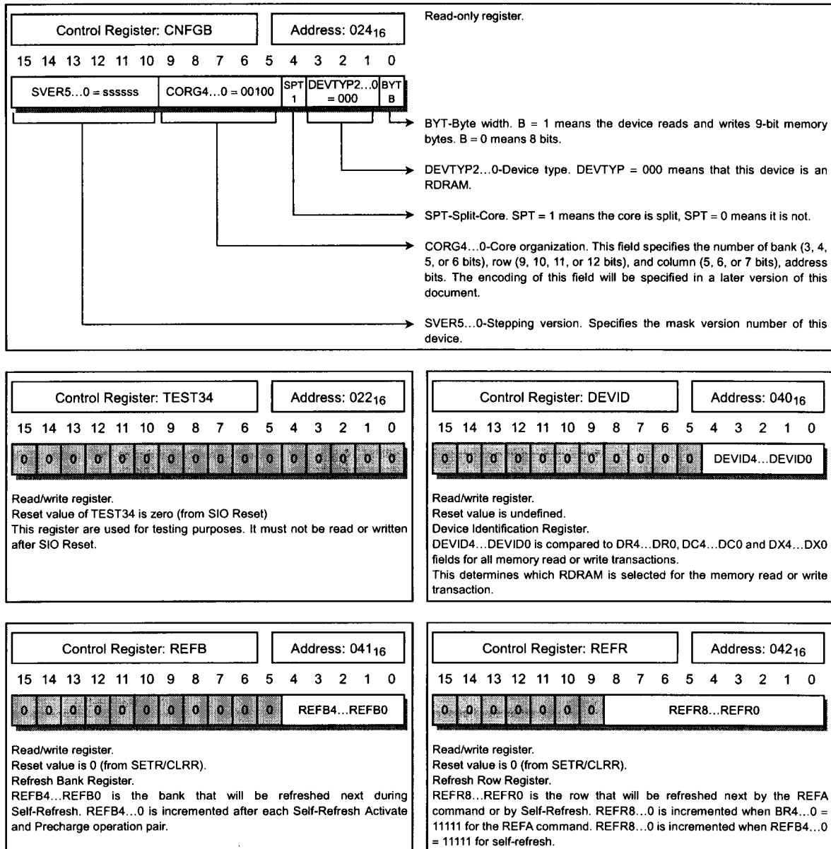
Figure 29. Control Registers
