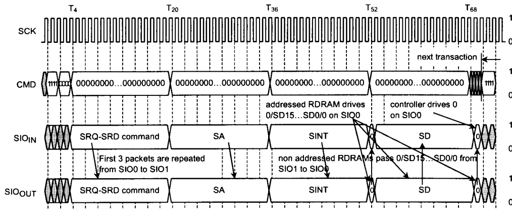
Figure 25. Serial Read (SRD) Transaction to Control Register
