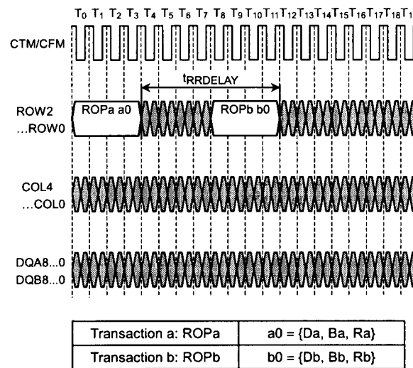
Figure 7. ROW-to-ROW Packet interaction-Timing
