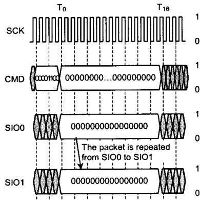
Figure 27. SIO Reset Sequence
