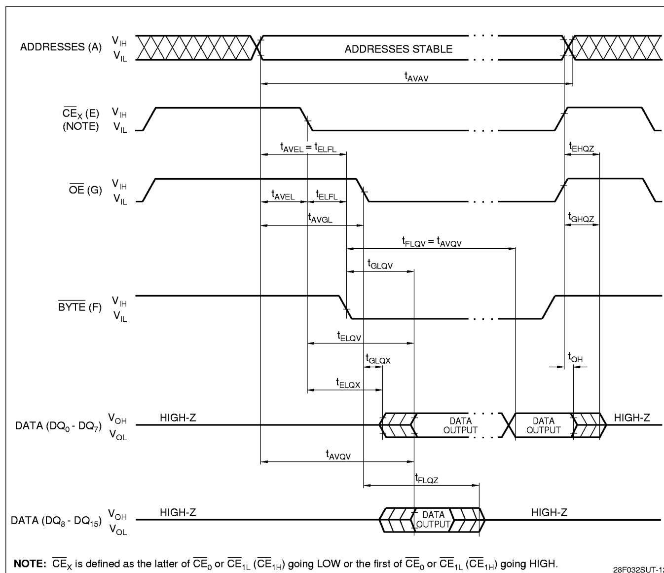
Figure 12. \overline{\text{BYTE}} Timing Waveforms
