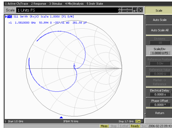
Smith Chart
