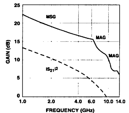
Figure 3. Insertion Power Gain, Maximum Available Gain and Maximum Stable Gain vs. Frequency. V_{DS} = 9\ \text{V} , I_{DS} = 125\ \text{mA} .
