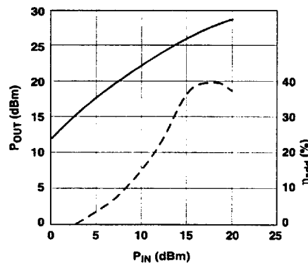
Figure 2. Output Power and Power Added Efficiency vs. Input Power. V_{DS} = 9\ \text{V} , I_{DS} = 125\ \text{mA} , f = 4.0\ \text{GHz} .
