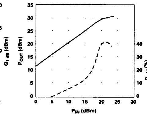
Figure 2. Output Power and Power Added Efficiency vs. Input Power. V_{DS} = 9\text{ V} , I_{DS} = 250\text{ mA} , f = 4.0\text{ GHz} .
