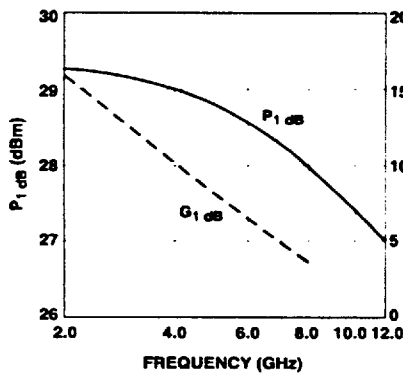
Figure 1. Power Output @ 1 dB Gain Compression and 1 dB Compressed Gain vs. Frequency. V_{DS} = 9\text{ V} , I_{DS} = 250\text{ mA} .
