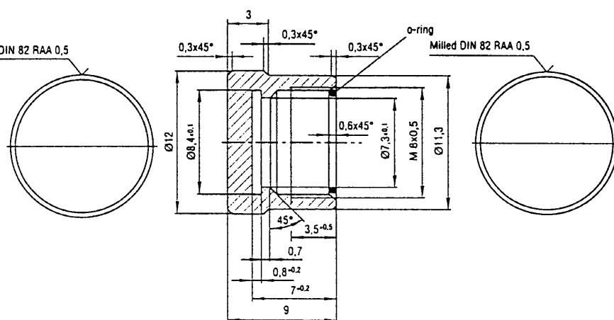
Dust cap: for pin connectors
