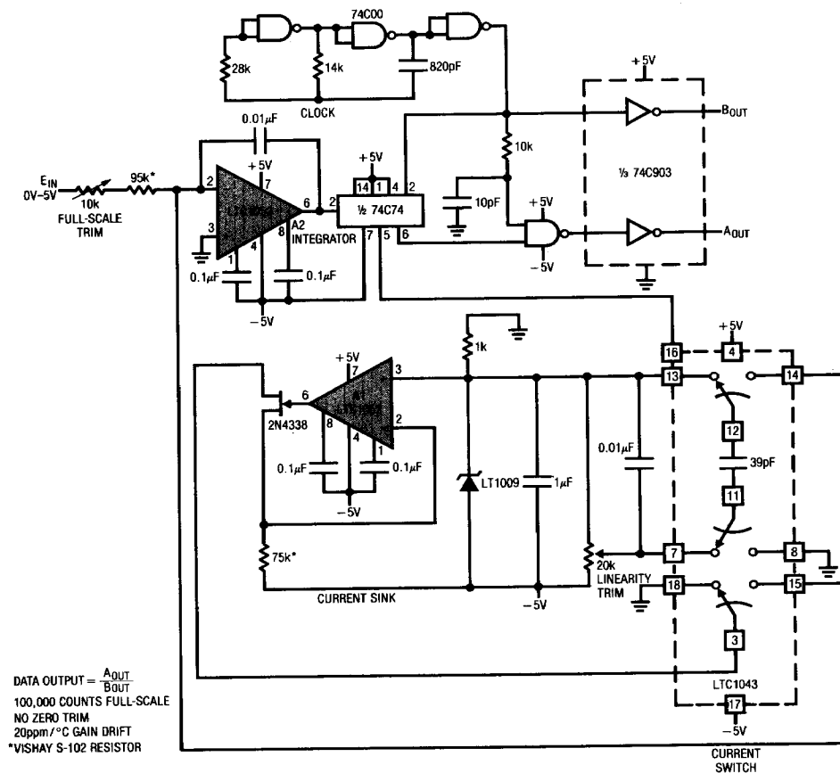
16-Bit A \rightarrow D Converter
