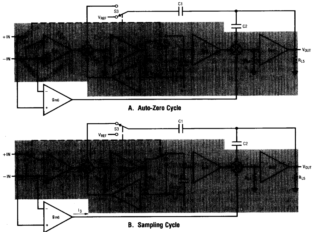
Figure 1. LTC1052 Block Diagram
