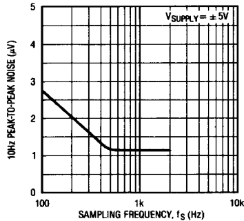
10Hzp-p Noise vs Sampling Frequency
