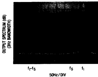
Aliasing Error
