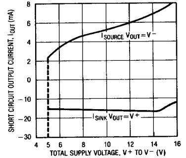
Output Short Circuit Current vs Supply Voltage
