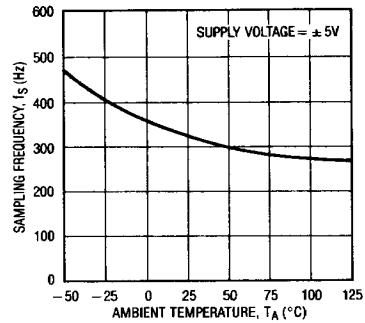
Sampling Frequency vs Temperature
