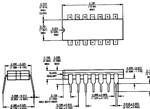
J Package 14-Lead Hermetic DIP
