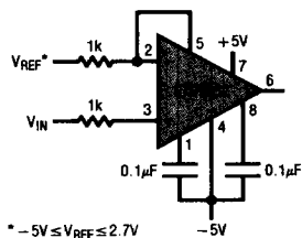
Comparator Operation
