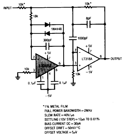
Fast Precision Inverter
