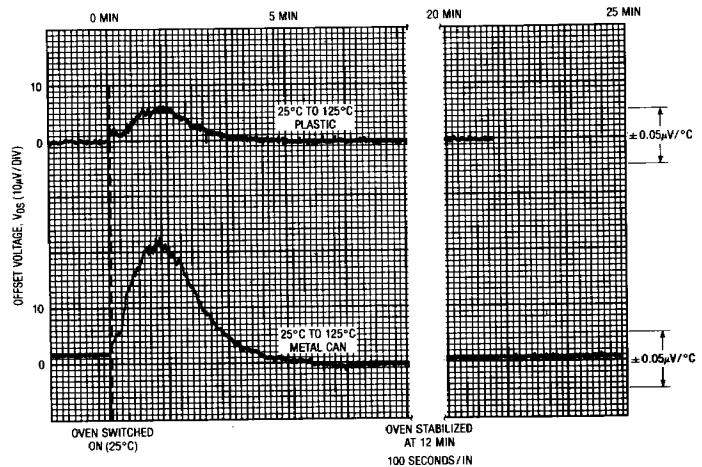
Figure 4. Transient Response of Offset Drift Test Circuit with 100°C Temperature Step
