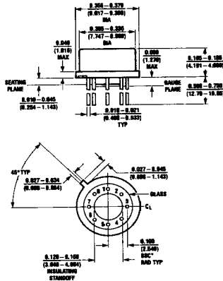
H Package Metal Can
