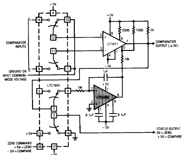
Offset Stabilized Comparator
