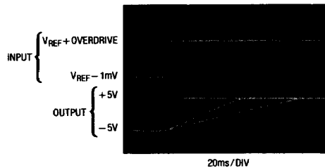
Response Time vs Overdrive
