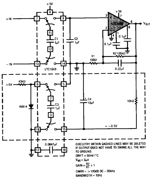
5V Powered Ultra Precision Instrumentation Amplifier
