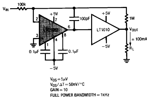
± 100mA Output Drive
