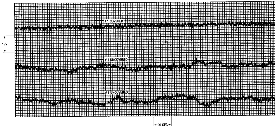
Figure 5. DC to 1Hz (Test Circuit TC3)
