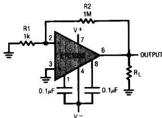
Electrical Characteristics Test Circuit (TC1)
