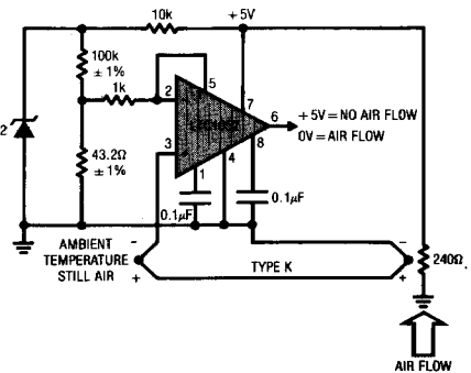
Air Flow Detector
