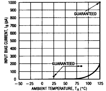
Input Bias Current vs Temperature
