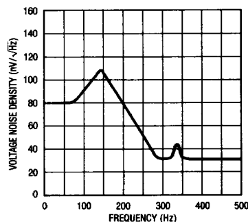
LTC1052 Noise Spectrum
