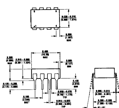
J8 Package 8 Lead Hermetic Dip
