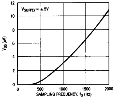
Offset Voltage vs Sampling Frequency
