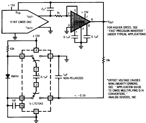
No V_{OS} Adjust* CMOS DAC Buffer—Single Supply
