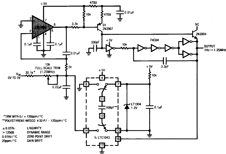
1Hz → 1.25MHz Voltage-to-Frequency Converter (+5V Supply)
