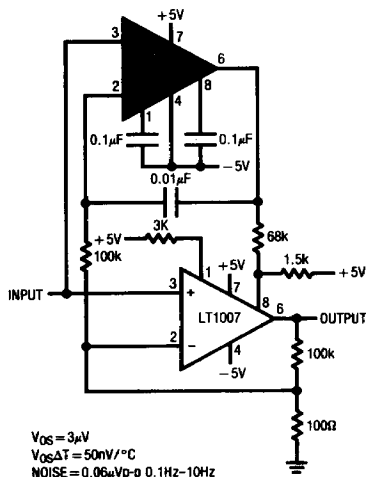
Ultra Low Noise, Low Drift Amplifier
