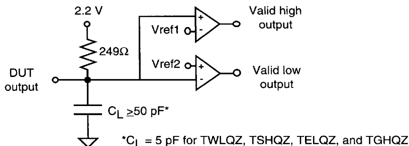
Tester Equivalent Load Circuit
