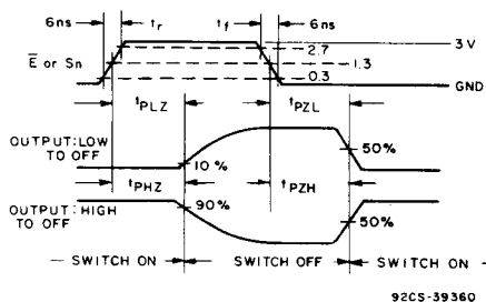
Fig. 21 - Switch propagation delay, turn-on, turn-off times.
