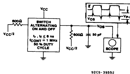
Fig. 12 - Control-to-switch feedthrough noise test circuit.
