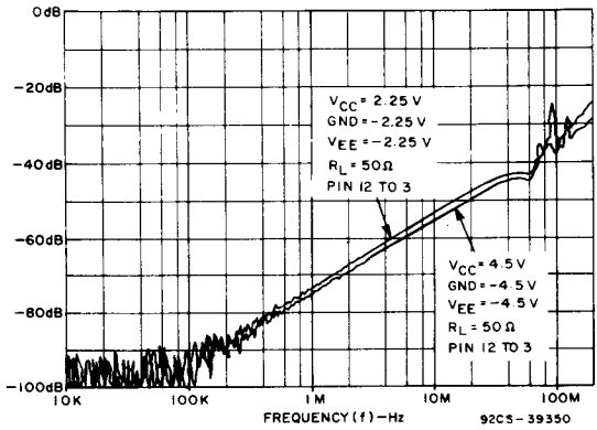
Fig. 15 - Channel off feedthrough (HC/HCT4351).
