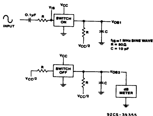
Fig. 10 - Crosstalk between two switches test circuit.
