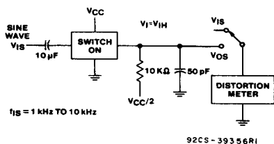
Fig. 11 - Sine wave distortion test circuit.
