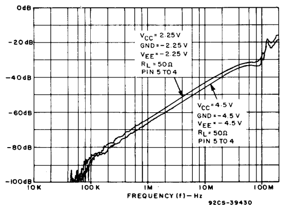
Fig. 19 - Channel off feedthrough (HC/HCT4353).
