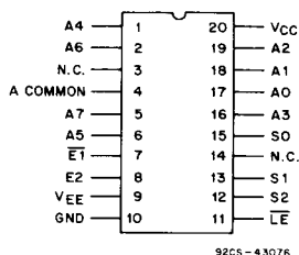
CD54/74HC/HCT4351 TERMINAL ASSIGNMENT
