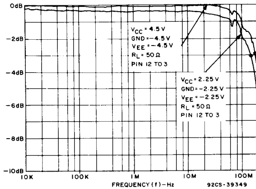
Fig. 14 - Channel on bandwidth (HC/HCT4351).
