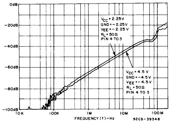
Fig. 17 - Channel off feedthrough (HC/HCT4352).
