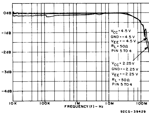
Fig. 18 - Channel on bandwidth (HC/HCT4353).
