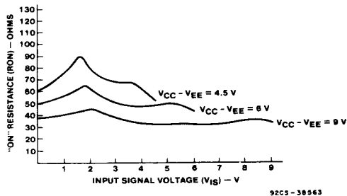
Fig. 20 - Typical ON resistance vs. input signal voltage.
