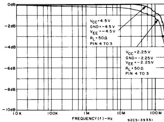
Fig. 16 - Channel on bandwidth (HC/HCT4352).
