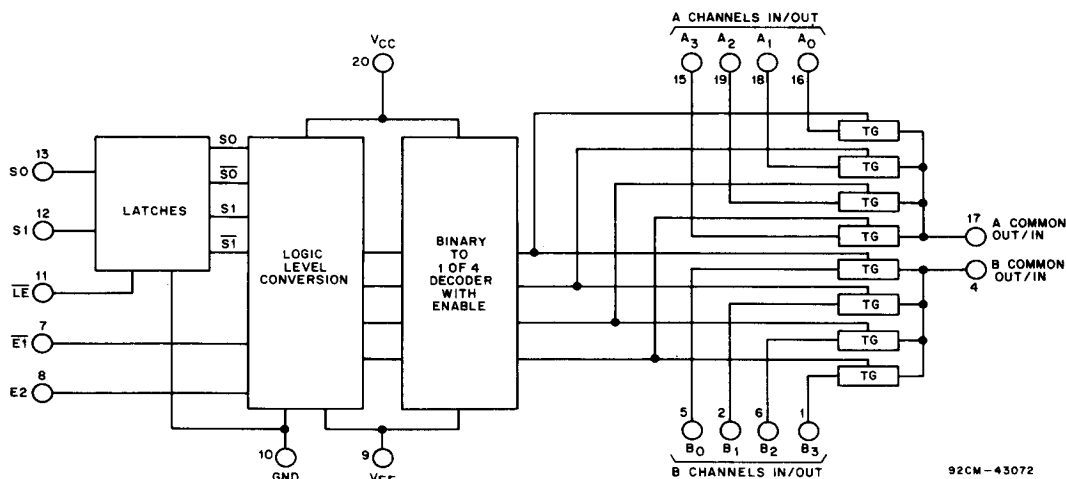
Fig. 3 - Functional diagram of HC/HCT4352.
