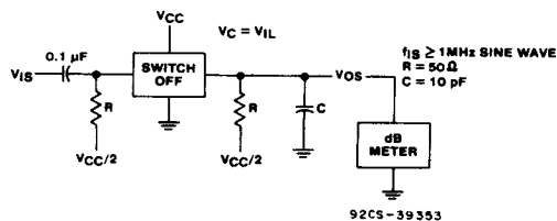
Fig. 13 - Switch off signal feedthrough.
