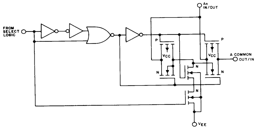
Fig. 2 - Detail of one HC/HCT4351 switch.
