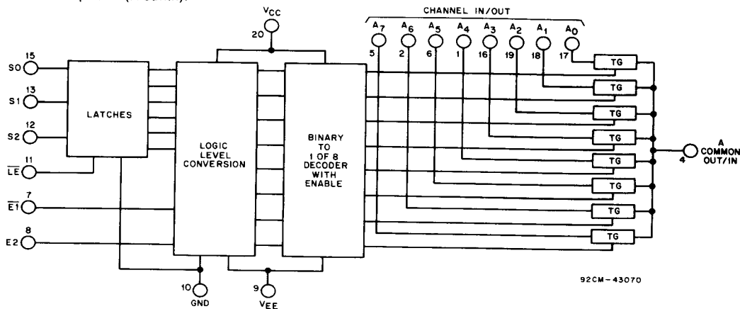
Fig. 1 - Functional diagram of HC/HCT4351.
