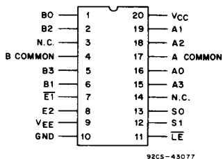
CD54/74HC/HCT4352 TERMINAL ASSIGNMENT
