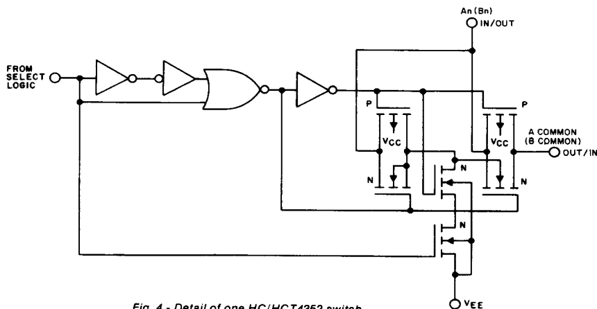
Fig. 4 - Detail of one HC/HCT4352 switch.
