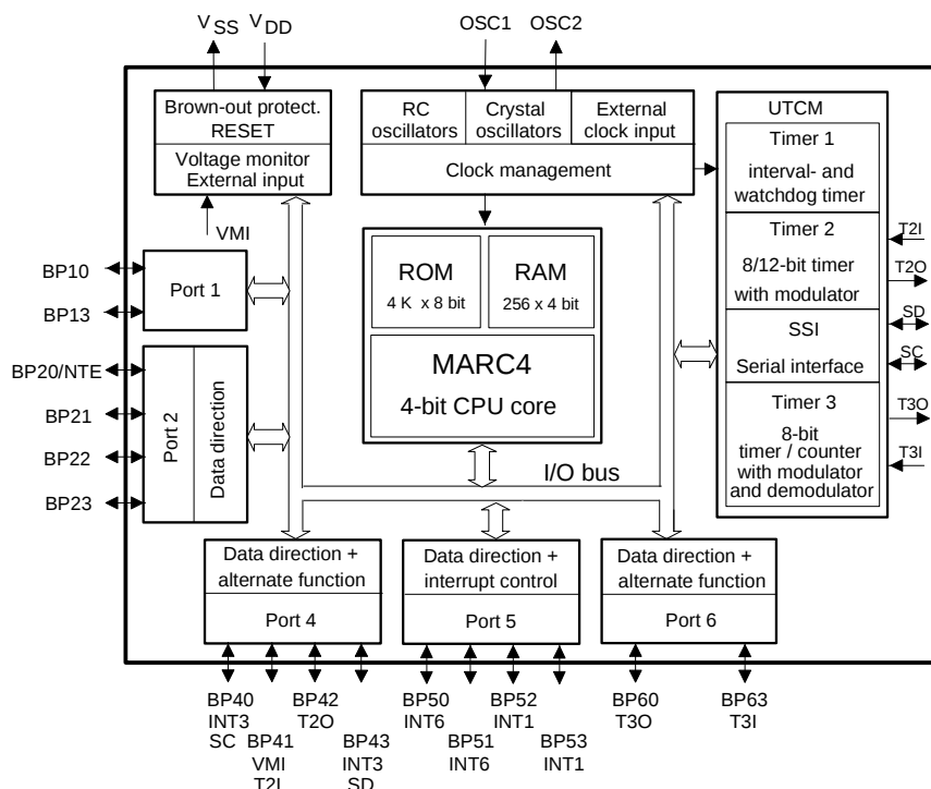
Figure 9. Block Diagram
