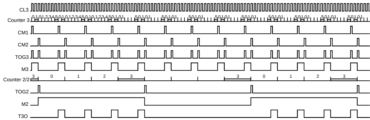
Figure 89. Burst Modulation 1
