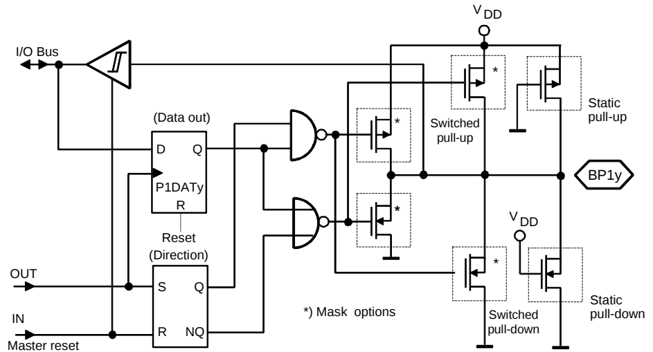
Figure 29. Bi-directional Port 1
