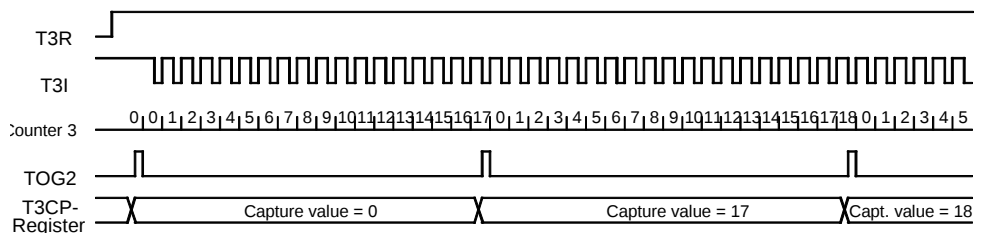
Figure 87. Frequency Measurement
