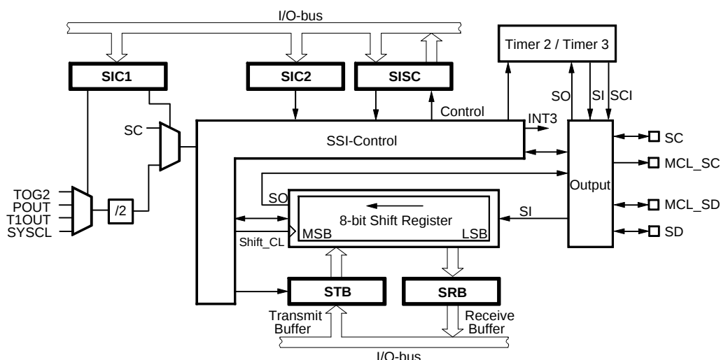
Figure 65. Block Diagram of the Synchronous Serial Interface
