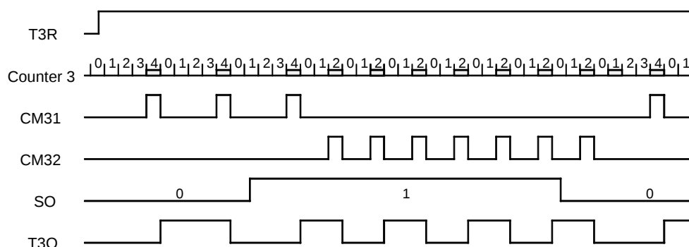
Figure 92. FSK Modulation
