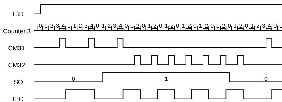
Figure 58. FSK Modulation
