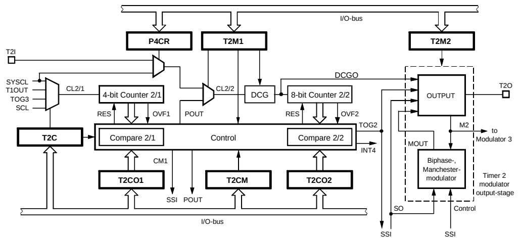
Figure 37. Timer 2
