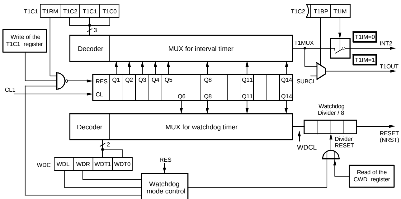
Figure 36. Timer 1 and Watchdog
