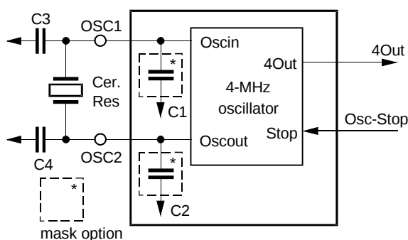
Figure 26. Ceramic Resonator
