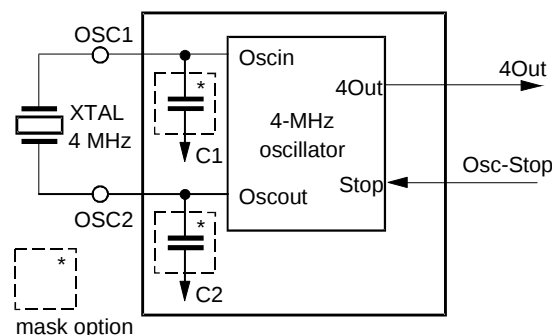
Figure 25. 4-MHz Crystal Oscillator
