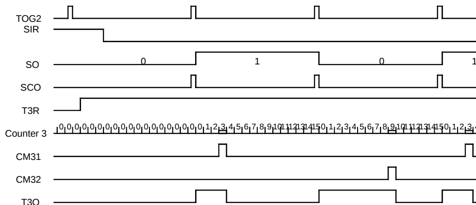
Figure 59. Pulse-width Modulation
