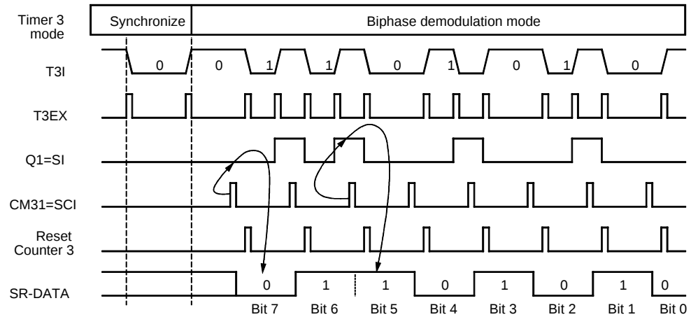
Figure 85. Biphase Demodulation
