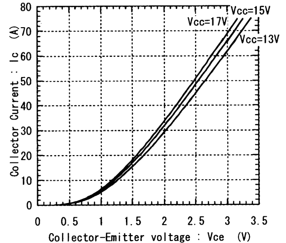
Collector current vs. Collector-Emitter voltage T_j=125^\circ\text{C} (Terminal)
