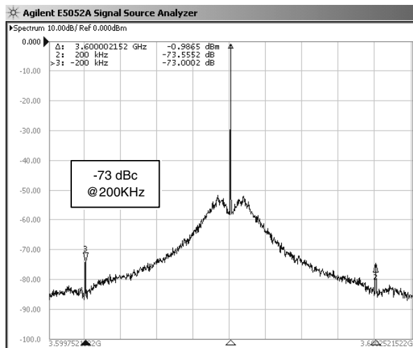
Figure 13. PFD Frequency Spurs (Div. by 4 Output; F_{\text{PFD}}=800\text{KHz} )
