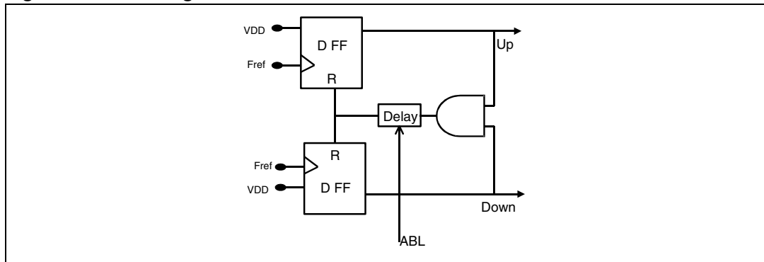
Figure 17. PFD diagram
