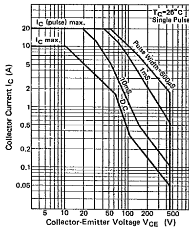
FORWARD BIAS SAFE OPERATING AREA
