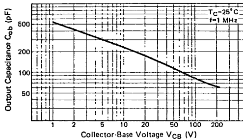
OUTPUT CAPACITANCE
