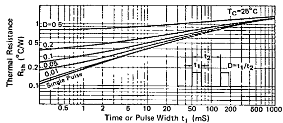
THERMAL RESPONSE
