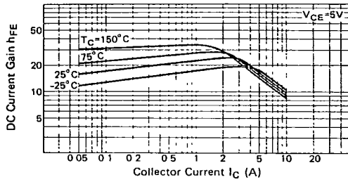
DC CURRENT GAIN
