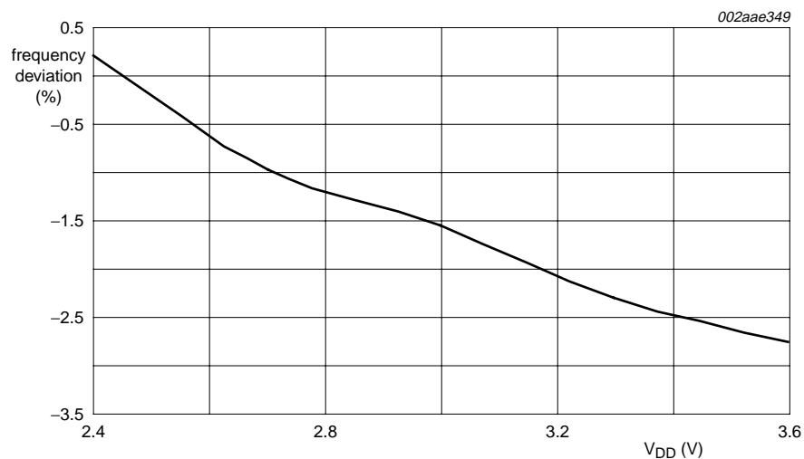
Fig 28. Average watchdog oscillator frequency vs. V_{DD} at -40\text{ }^{\circ}\text{C}
