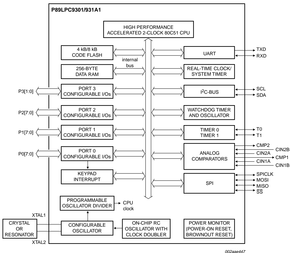
Fig 1. Block diagram
