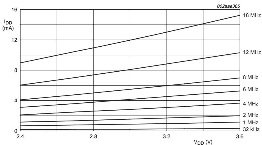
Fig 18. I_{DD(oper)} vs. frequency at +85 °C
