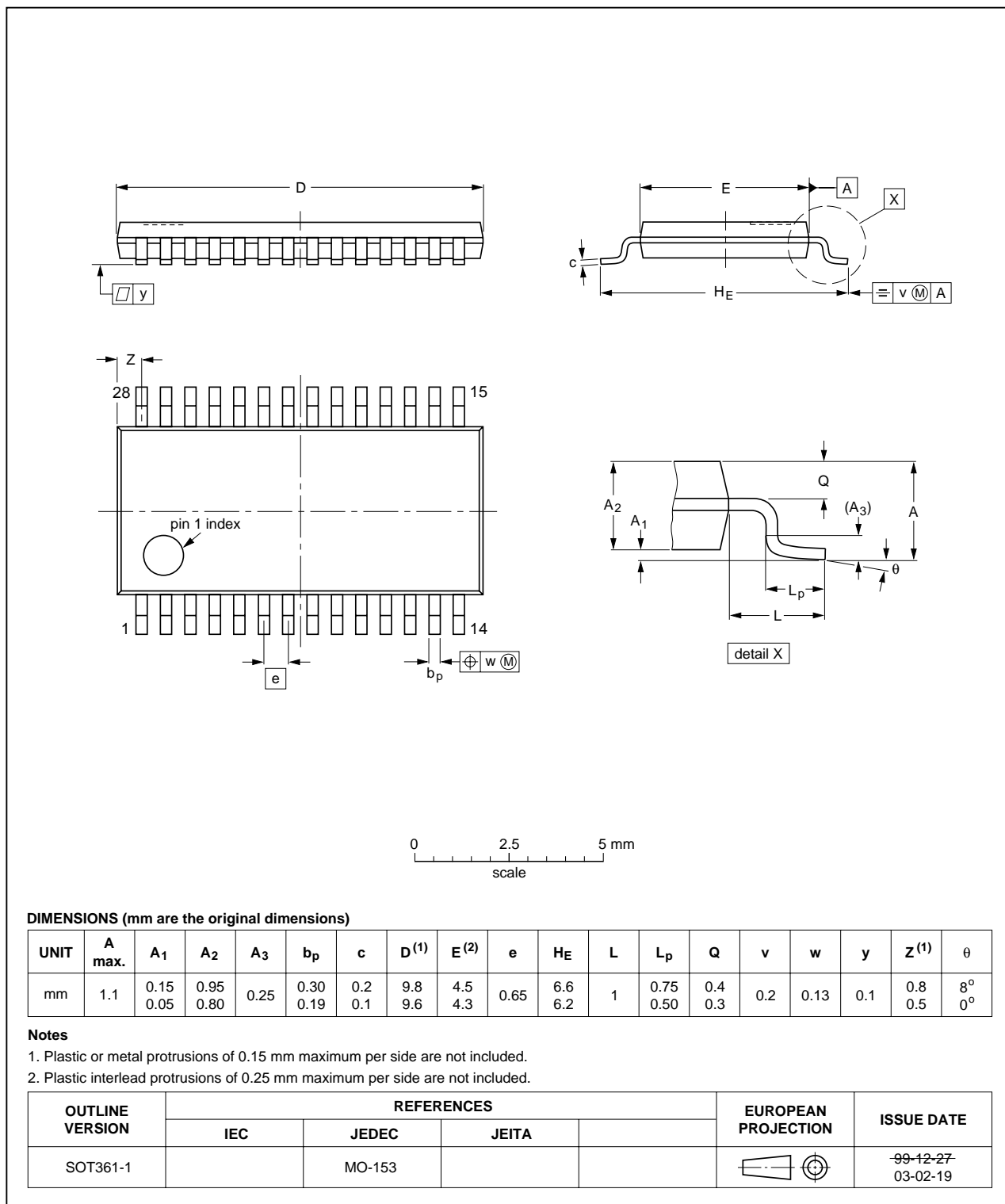
Fig 38. TSSOP package outline (SOT361-1)
