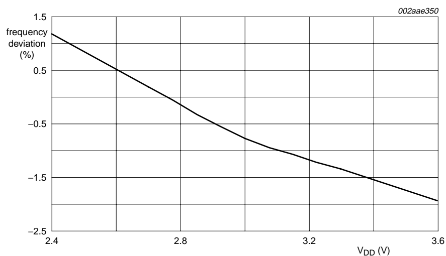
Fig 29. Average watchdog oscillator frequency vs. V_{DD} at +85\text{ }^{\circ}\text{C}
