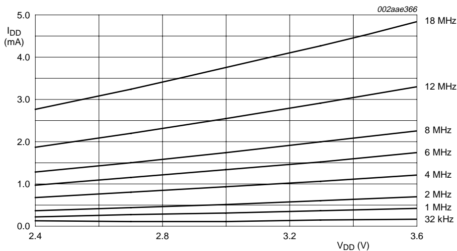
Fig 19. I_{DD(idle)} vs. frequency at +25 °C
