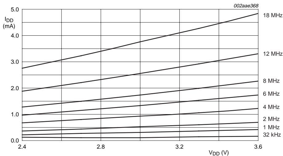
Fig 21. I_{DD(idle)} vs. frequency at +85\text{ }^{\circ}\text{C}
