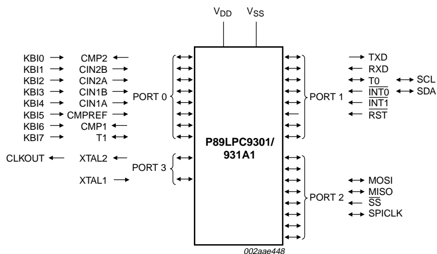
Fig 2. Functional diagram
