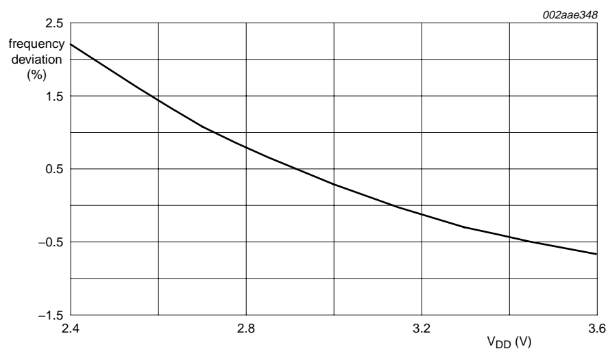
Central frequency of watchdog oscillator = 400 kHz Fig 27. Average watchdog oscillator frequency vs. V_{DD} at +25 °C
