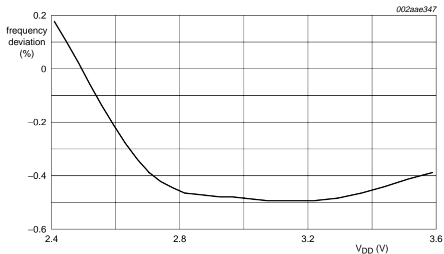
Central frequency of internal RC oscillator = 7.3728 MHz Fig 26. Average internal RC oscillator frequency vs. V_{DD} at +85 °C
