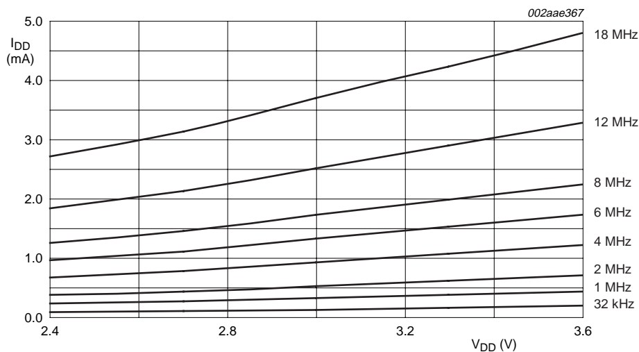
Fig 20. I_{DD(idle)} vs. frequency at -40\text{ }^{\circ}\text{C}
