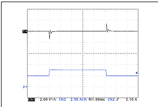
Figure 5: Output voltage response to step-change in load current (50%-75%-50% of Iout(max)); dI/dt = 0.05 A/ \mu s. Load cap: 1 \mu F ceramic capacitor. Ch 1: Vout (2 V/div), Ch 2: Iout (2.5 A/div).
