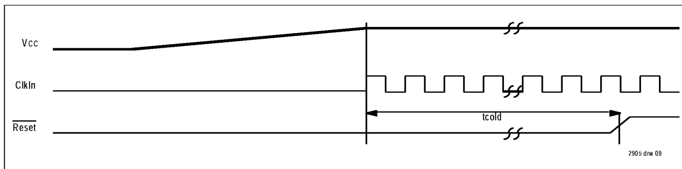
Figure 3: Power-On Reset Sequence
