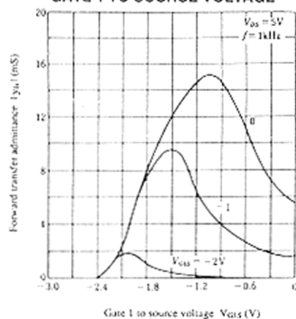
FORWARD TRANSFER ADMITTANCE VS. GATE 1 TO SOURCE VOLTAGE
