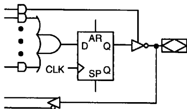
Registered Active-Low I/O
