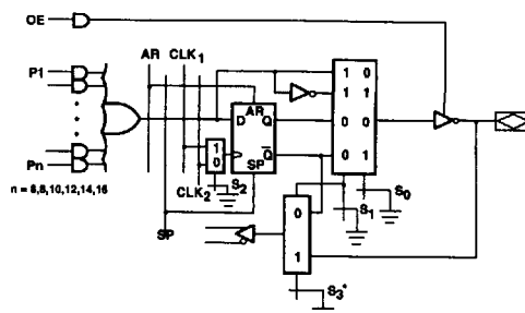
Figure 1. PALCE26V12 Macrocell
