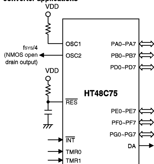
RC oscillator for multiple I/O and D/A converter applications
