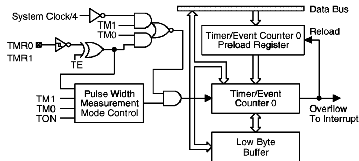
Timer/event counter 0/1
