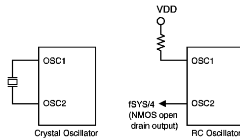
System oscillator
