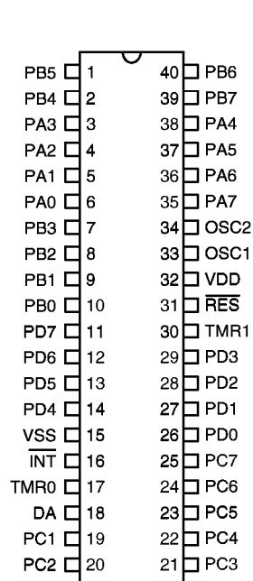
HT48C75 - 40 DIP-B-0
