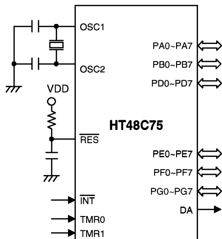
Crystal oscillator or ceramic resonator for multiple I/O and D/A converter applications
