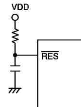
Reset circuit
