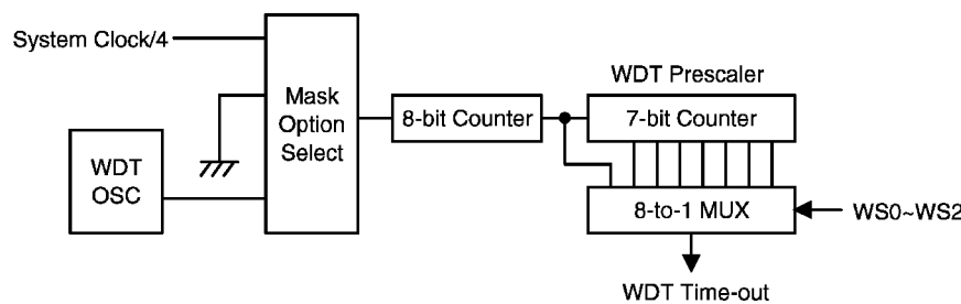
Watchdog timer
