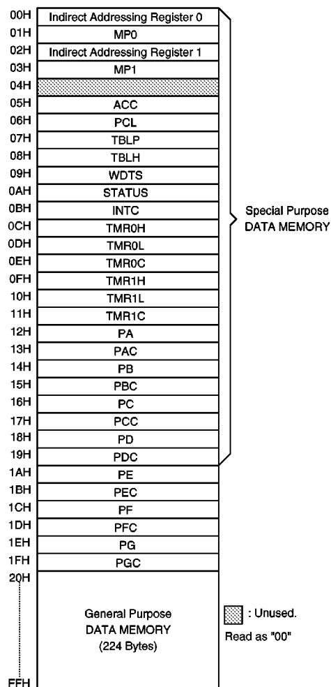
RAM mapping
