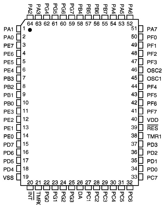
HT48C75 - 64 QFP-B-0
