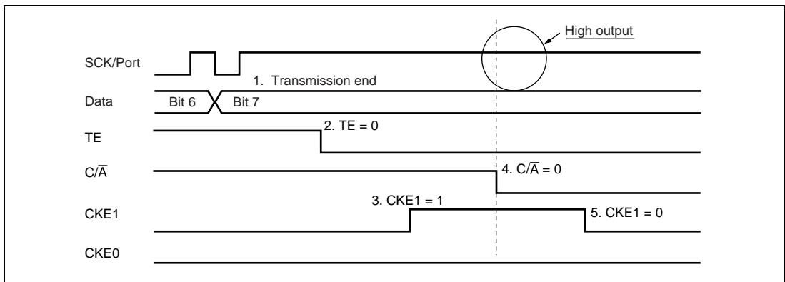
Figure 15.29 Prevention of Low Pulse Output at Switching from SCK Pins to Port Pins
