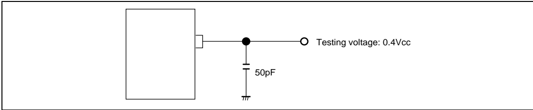
Figure 28.31 Tester Measurement Condition
