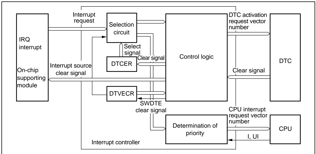
Figure 5.8 DTC and Interrupt Controller
