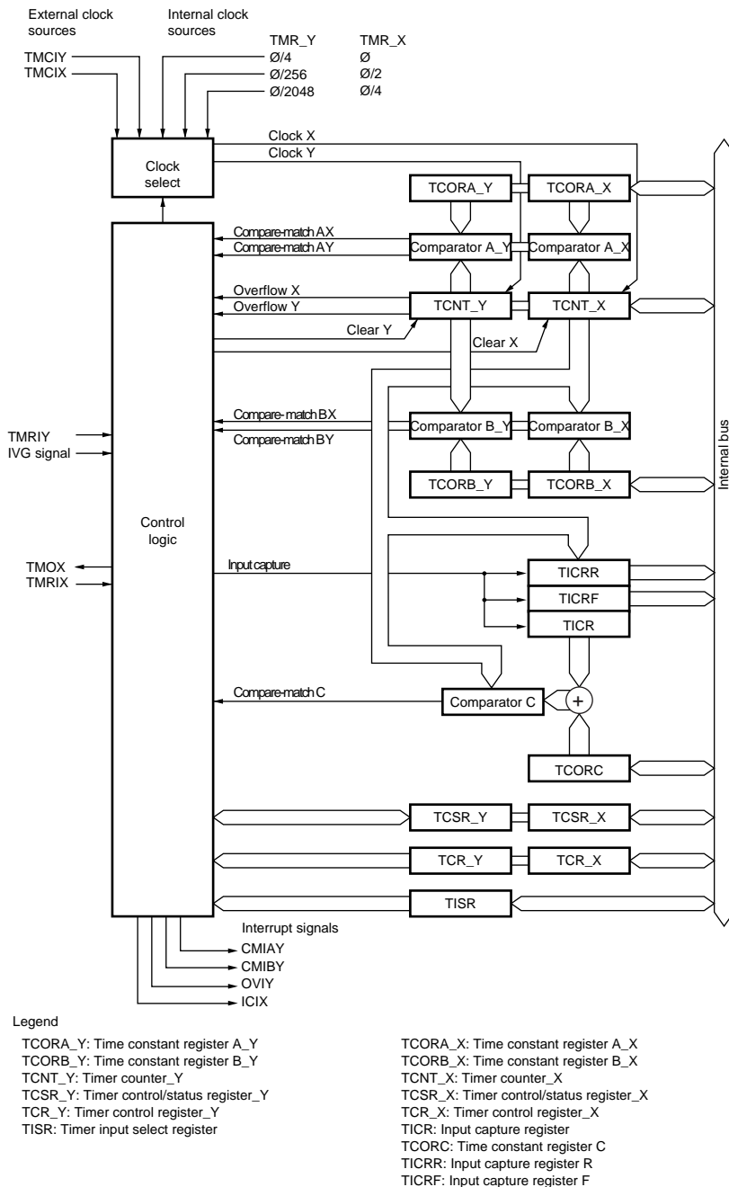
Figure 12.2 Block Diagram of 8-Bit Timers (TMR_Y and TMR_X)
