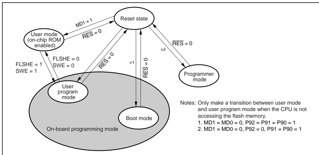
Figure 23.2 Flash Memory State Transitions
