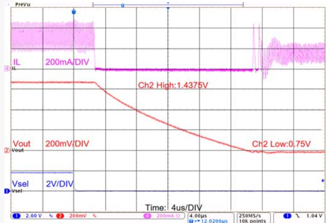
Figure 28. VSEL Transition, VSEL 1 to 0, R_{LOAD} = 4\Omega
