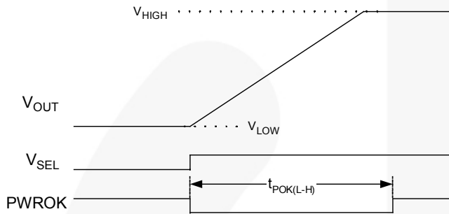
Figure 36. Multi-Step V_{OUT} Transition
