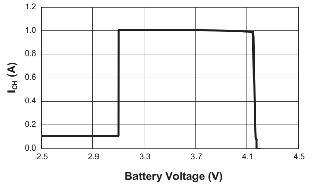
Adapter Charging Current vs. Battery Voltage ( R_{SETADP} = 8.06k\Omega )
