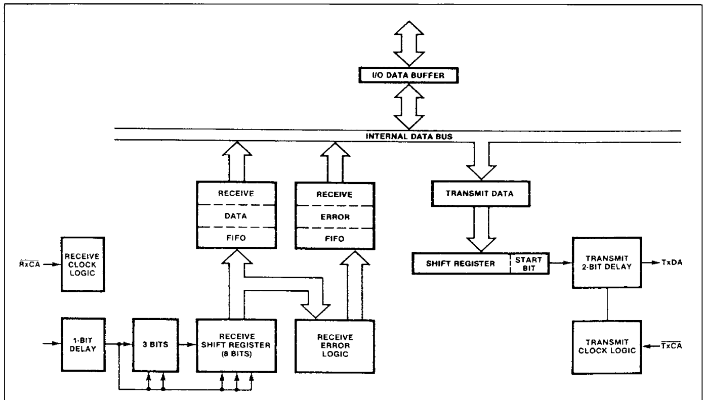
Figure 4 : Data Path.
