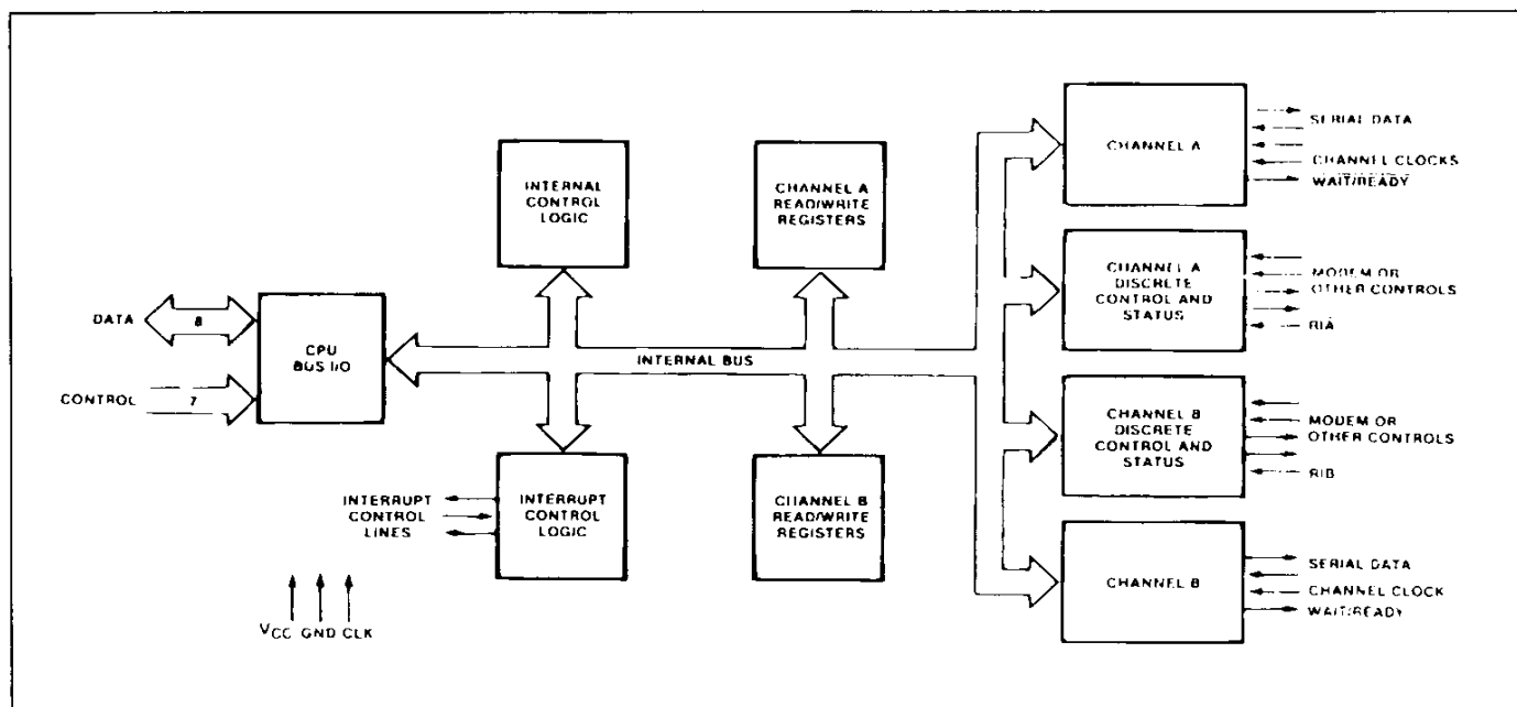
Figure 3 : Block Diagram.
