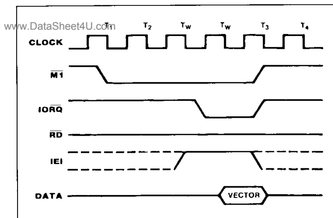
Figure 5c : Interrupt Acknowledge Cycle.
