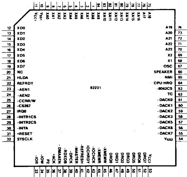
Pin Diagram 82231
