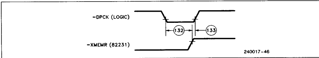
Figure 32. 82231 DPCK Timing
