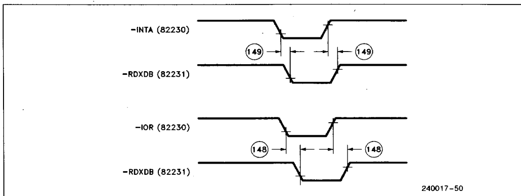
Figure 36. 82231 RDXDB Timing
