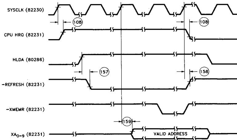
Figure 39. 82231 REFRESH Timing
