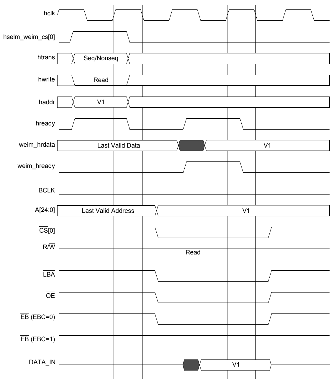
Figure 54. WSC = 1, A.HALF/E.HALF
